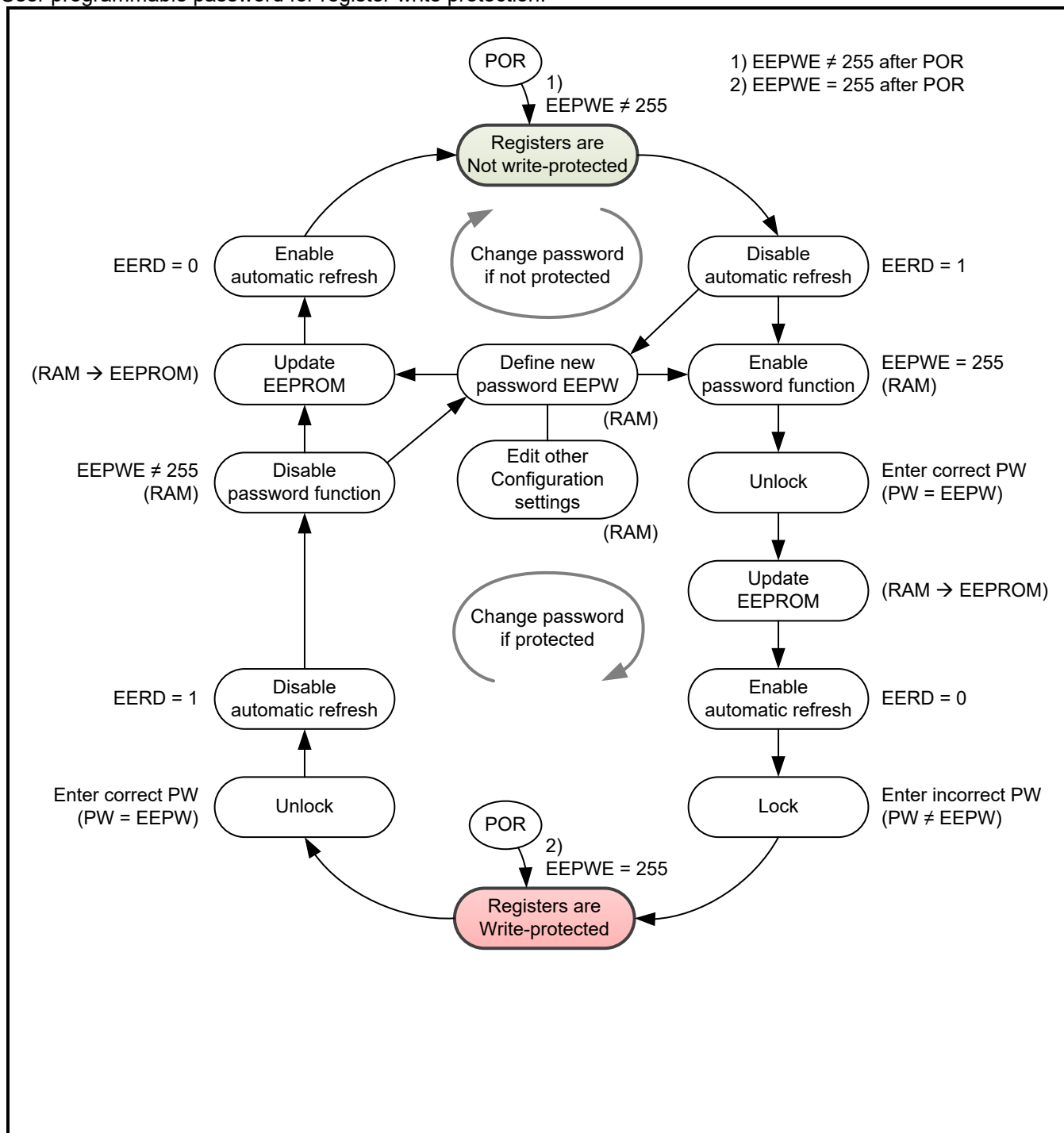
Figure 7-24 User Programmable Password Flowchart
