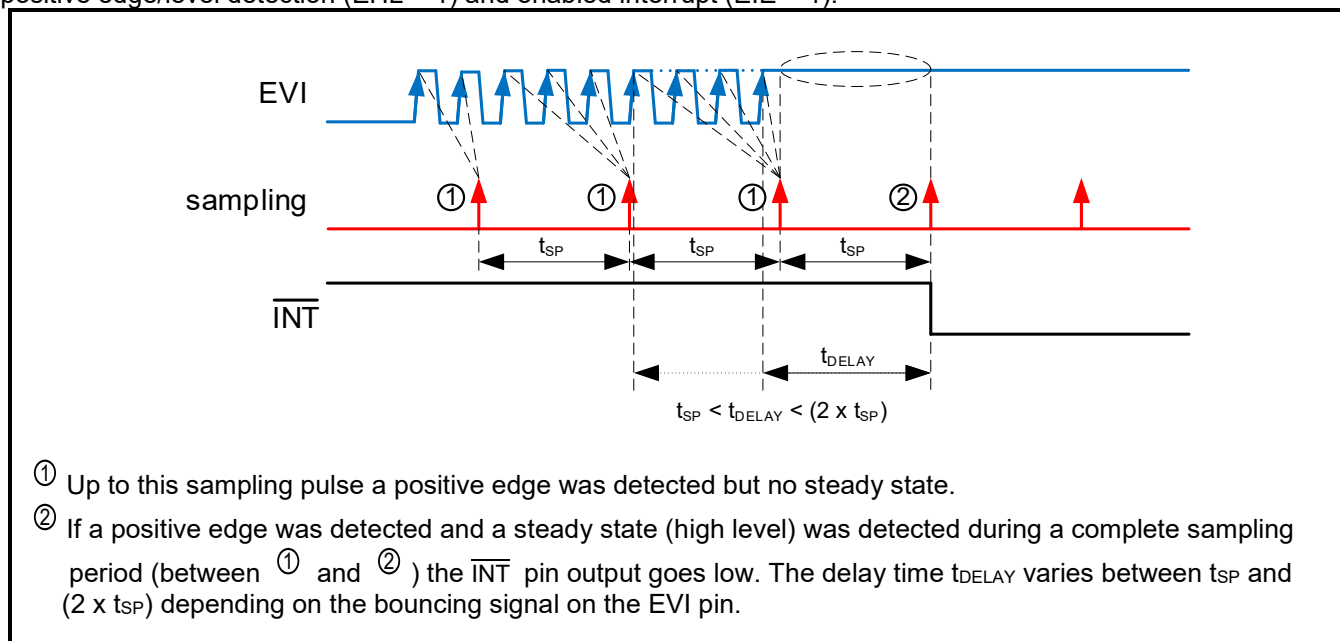
Figure 7-18 External Event function, with Filtering example, EIE = 1
