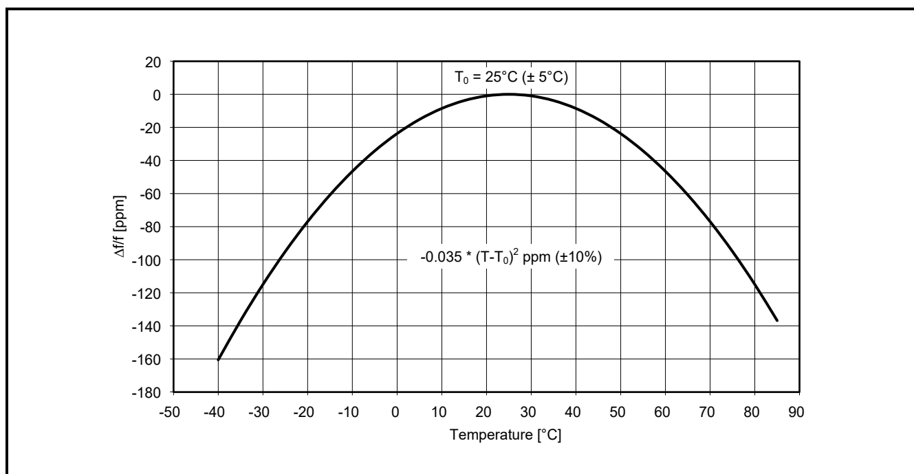
Figure 5-1 Xtal Frequency Characteristics
