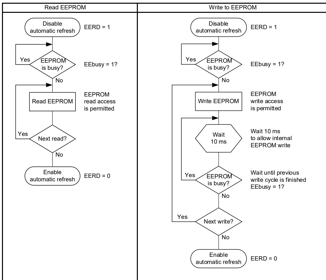
Figure 7-8 EEBusy bit
