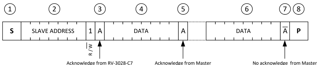
Figure 7-31 I 2 C Master reads data from slave EM3028 immediately after first byte
