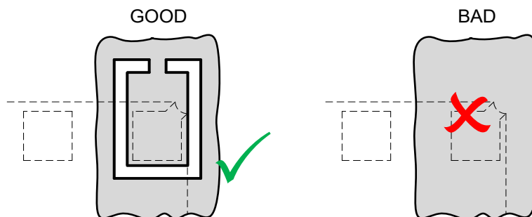
Figure 10-2 C7 Package Thermal Relief
