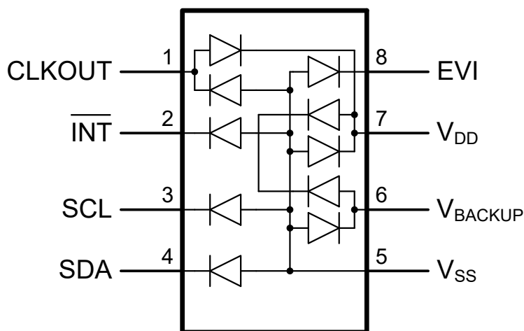
Figure 1-3 Device Diode Protection Diagram
