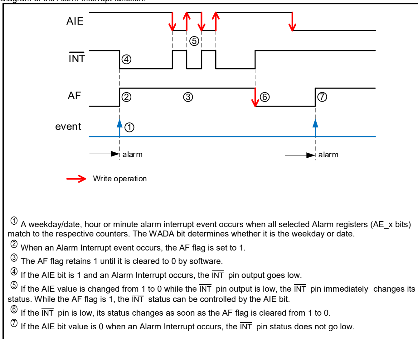
Figure 7-15 Alarm Interrupt
