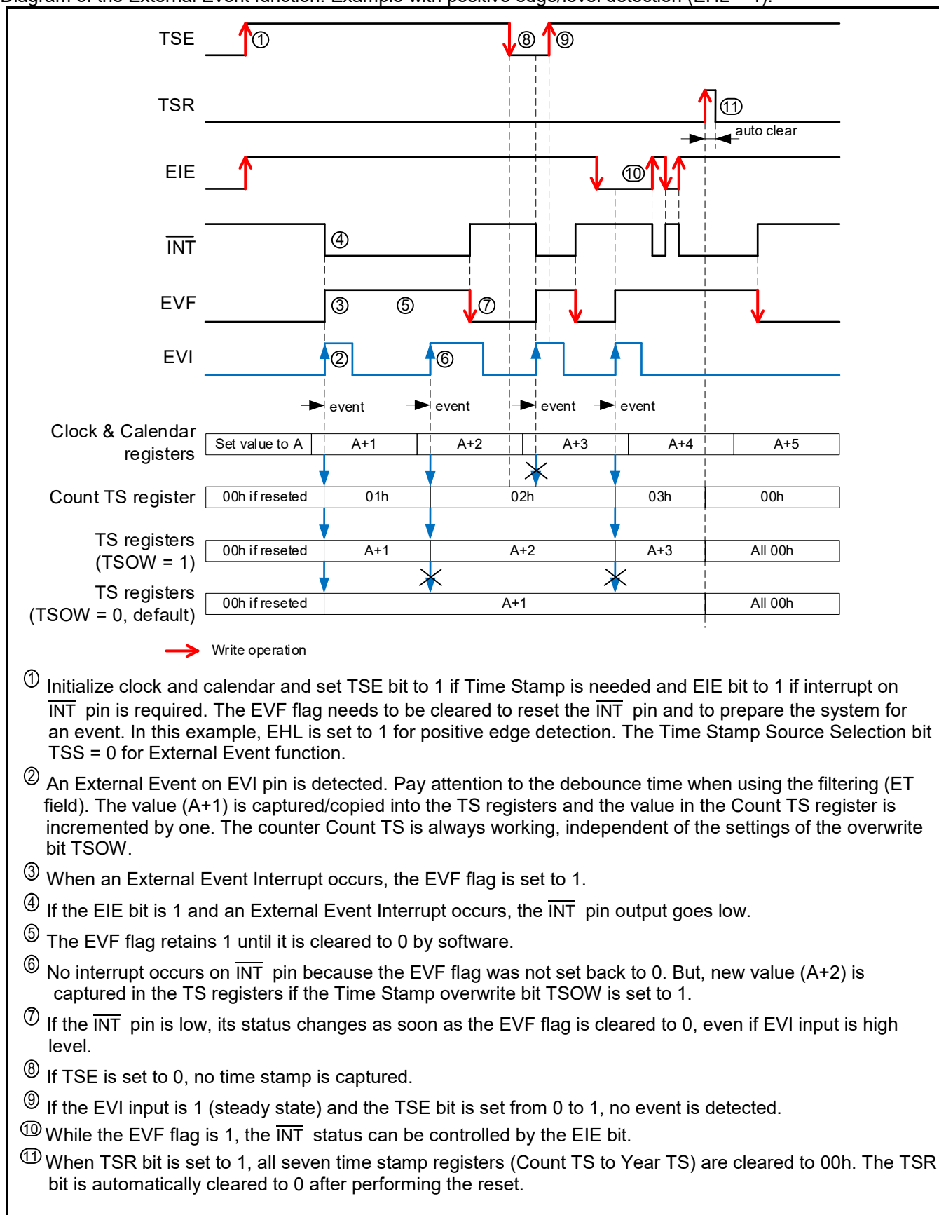
Figure 7-16 External Event
