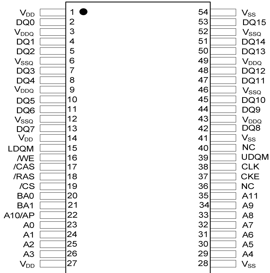
54pin TSOP-II / (400mil x 875mil) / (0.8mm Pin pitch)
