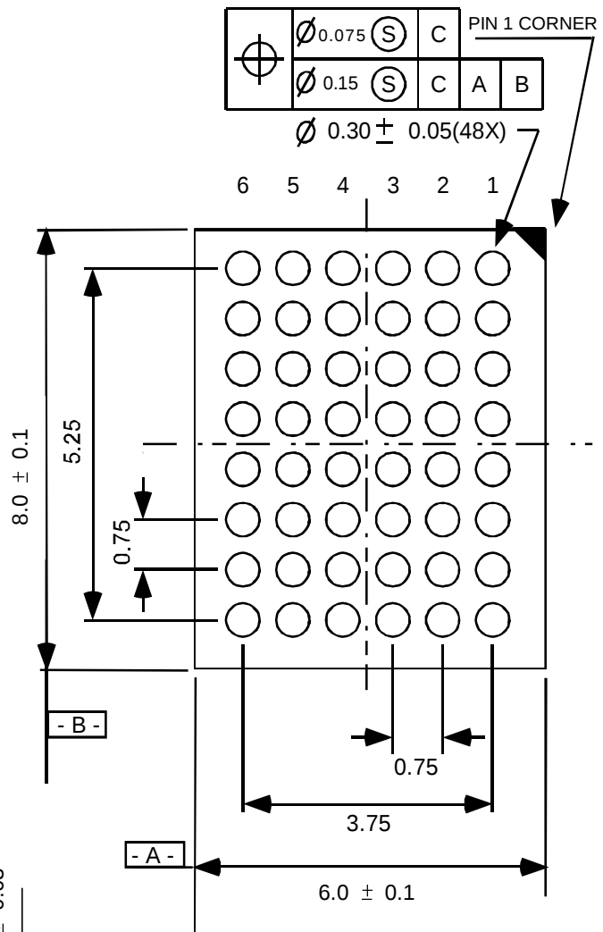
BOTTOM VIEW
