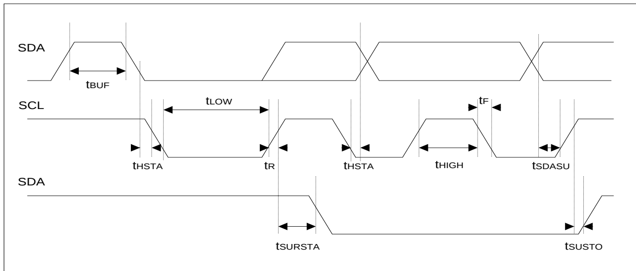
Figure 2 I²C timing diagram
