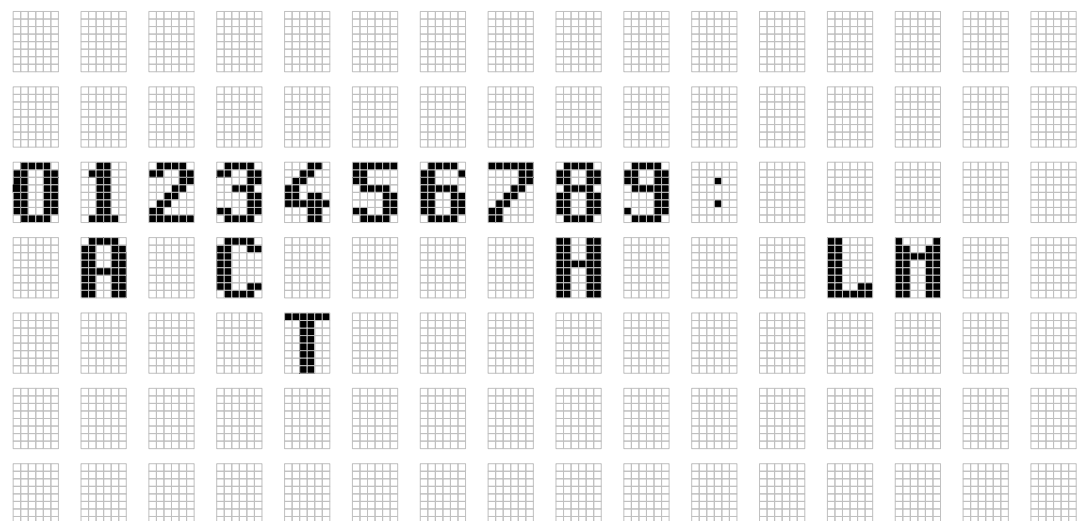
Figure 56 6x8 characters
