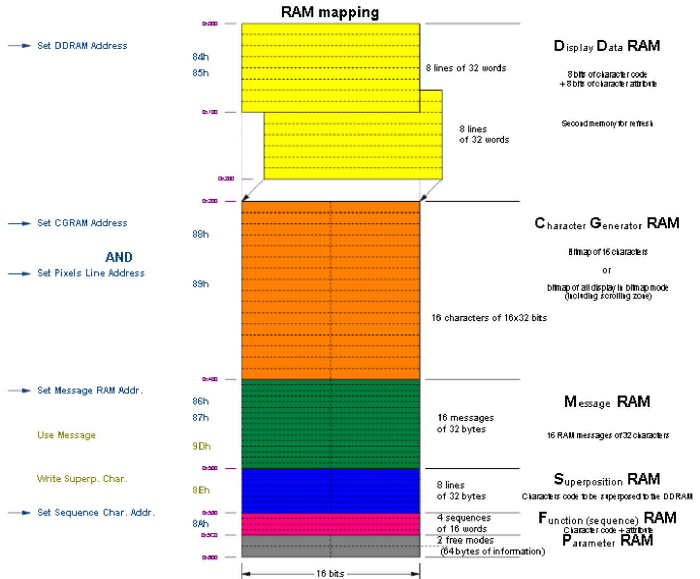
Figure 10 RAM Mapping
