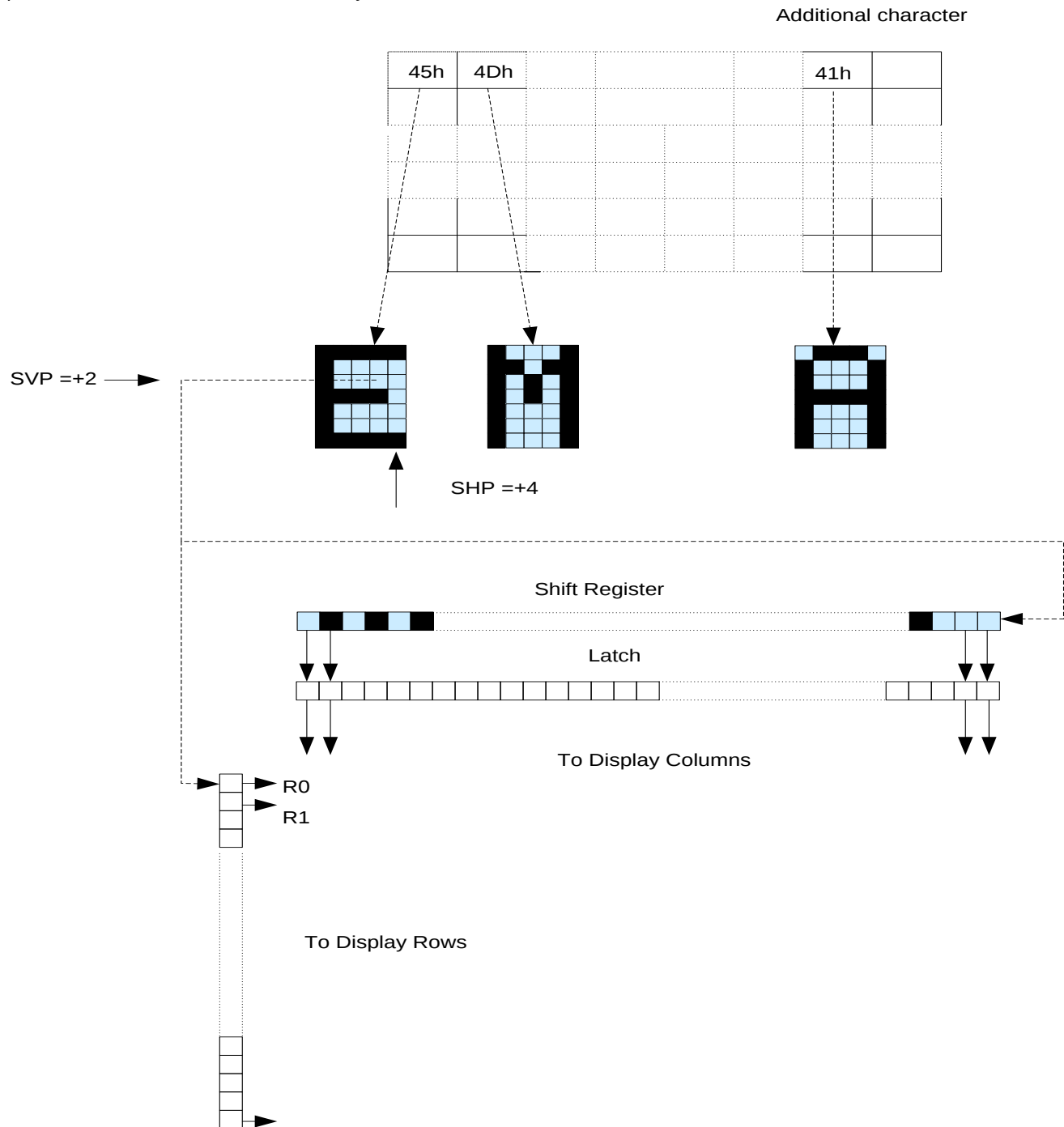
Figure 28 Scrolling function
