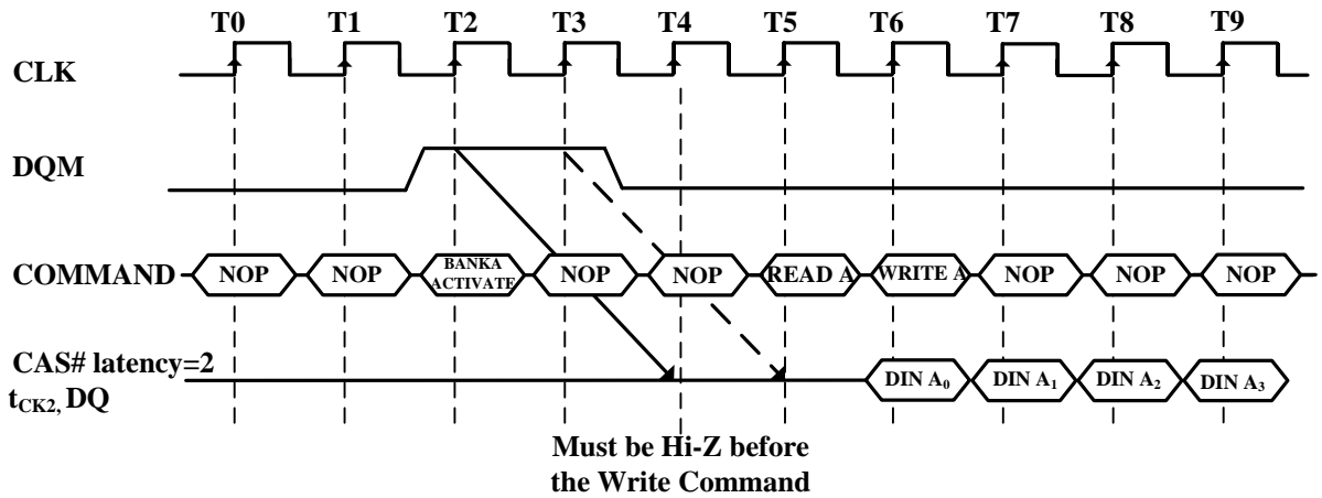
Figure 6. Read to Write Interval (Burst Length ≥ 4, CAS# Latency = 2)
