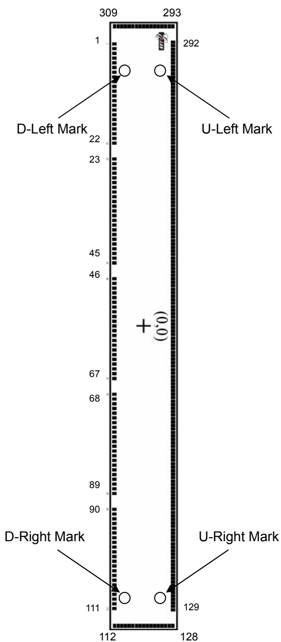
Fig. 1 Pin Configuration
