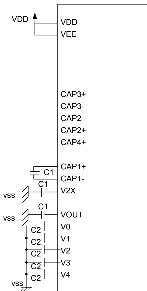
When using internal power circuit. (2 times boosting)
