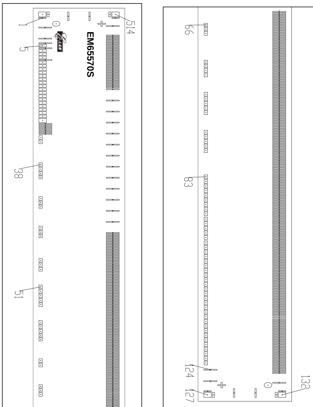
Figure 1 Pin Configuration
