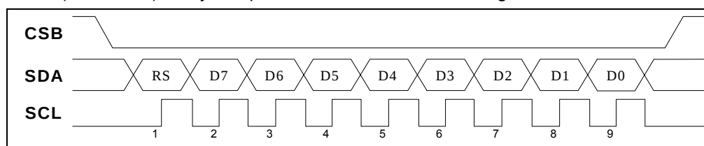
Figure 7-2 3-Wires Type Serial Interface
