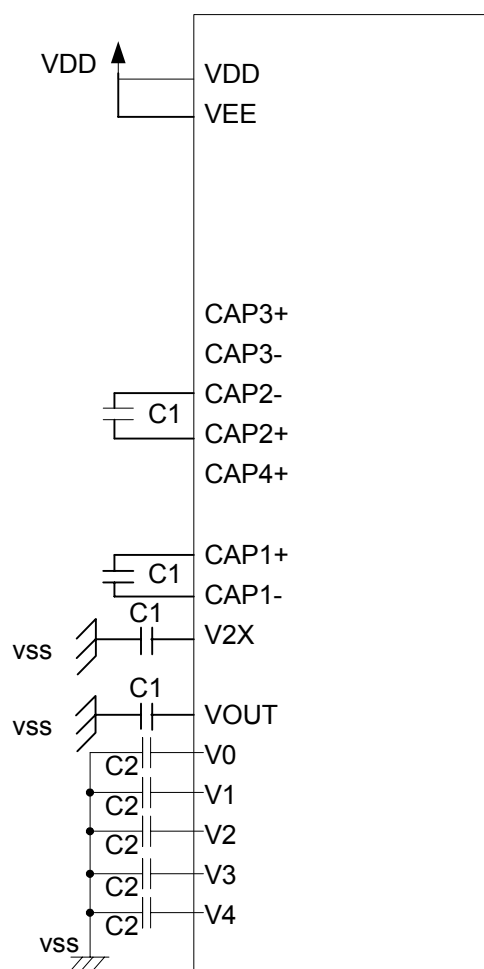
When using internal power circuit. (3 times boosting)
