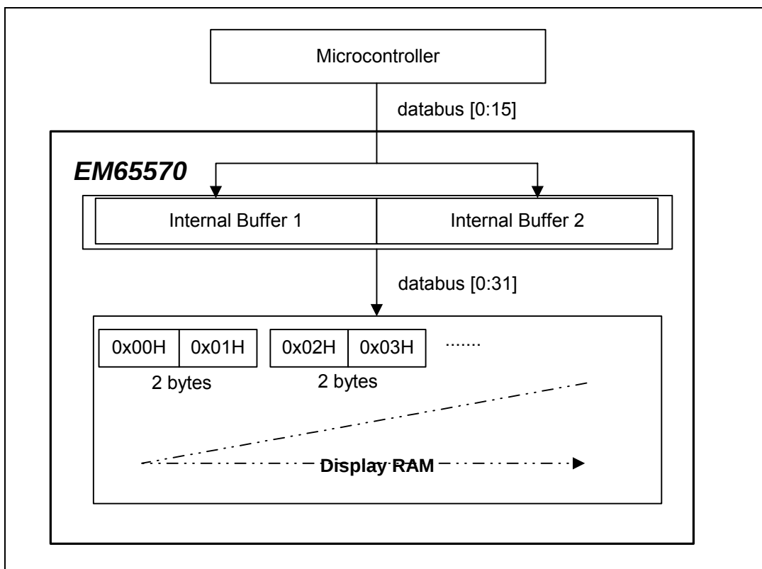
Figure 7-6 Burst RAM Write Operation
