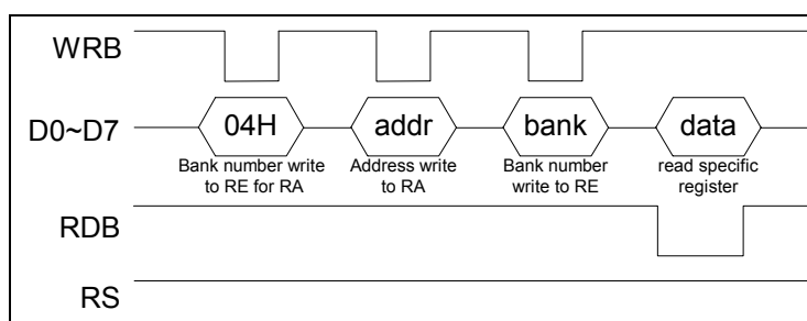
Figure 7-5 Register Read Operation
