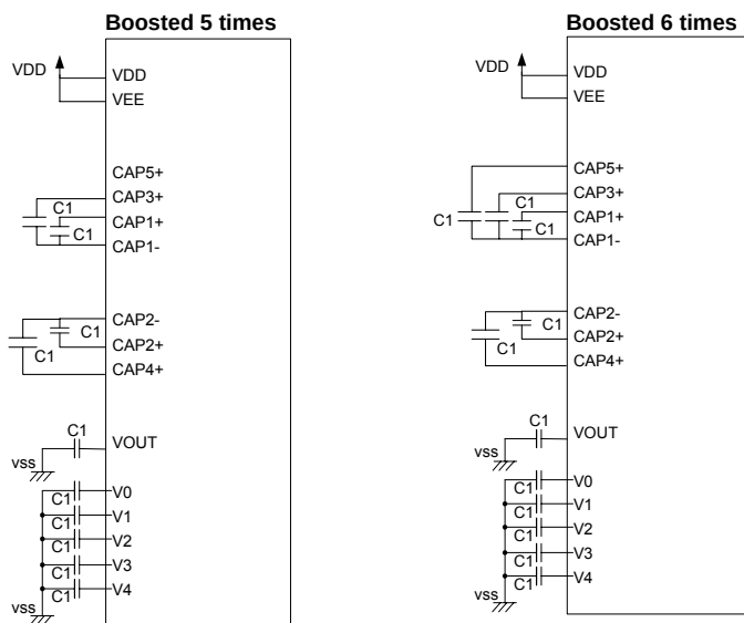
Figure 7-17b Internal Power Capacitor Connections Application Circuits (Voltage Boosted 5 and 6 Times)
