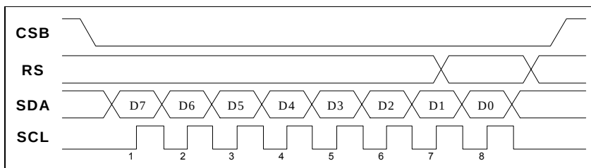
Figure 7-2 4-Wire Type Serial Interface
