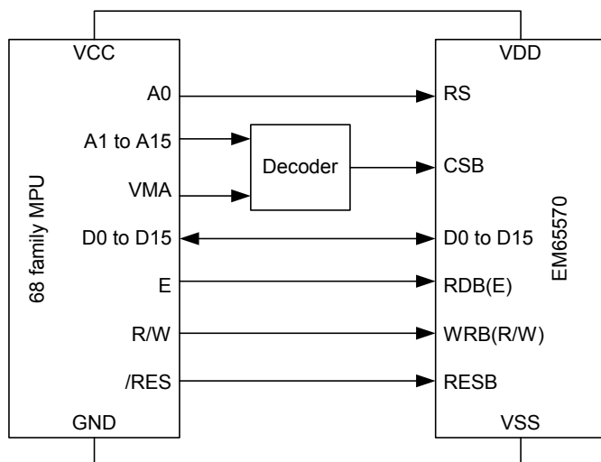
Figure 12-2 Connected to 68-Family MCU Application Circuit Diagram
