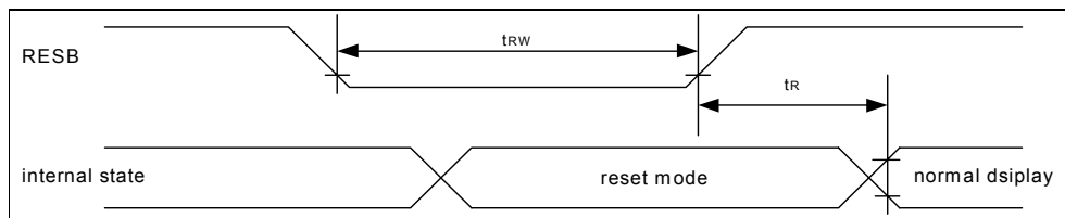
Figure 11-7 Reset Timing Diagram
