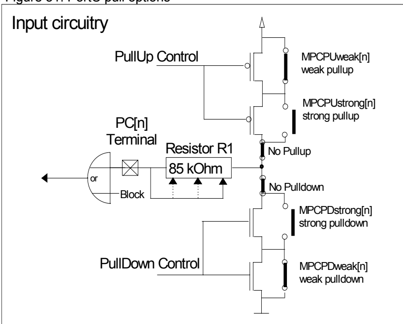
Figure 31. PortC pull options
