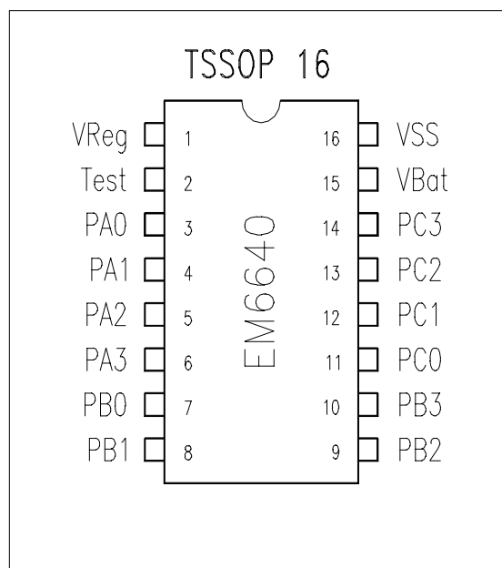
Figure 2 Pin Configuration of TSSOP16
