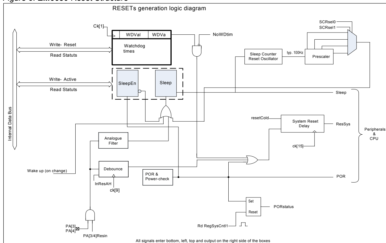
Figure 6. EM6680 Reset Structure
