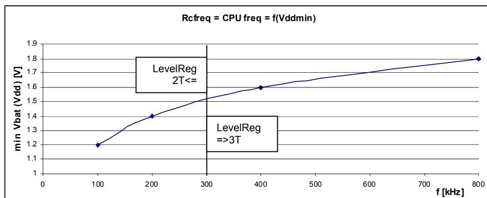
Figure 29. Minimum V_{DD} = f(RC \text{ oscillator})
