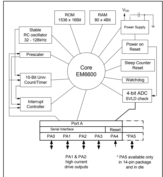
Figure 1. Architecture
