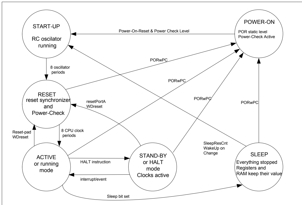
Figure 5. EM6680 operating mode transitions
