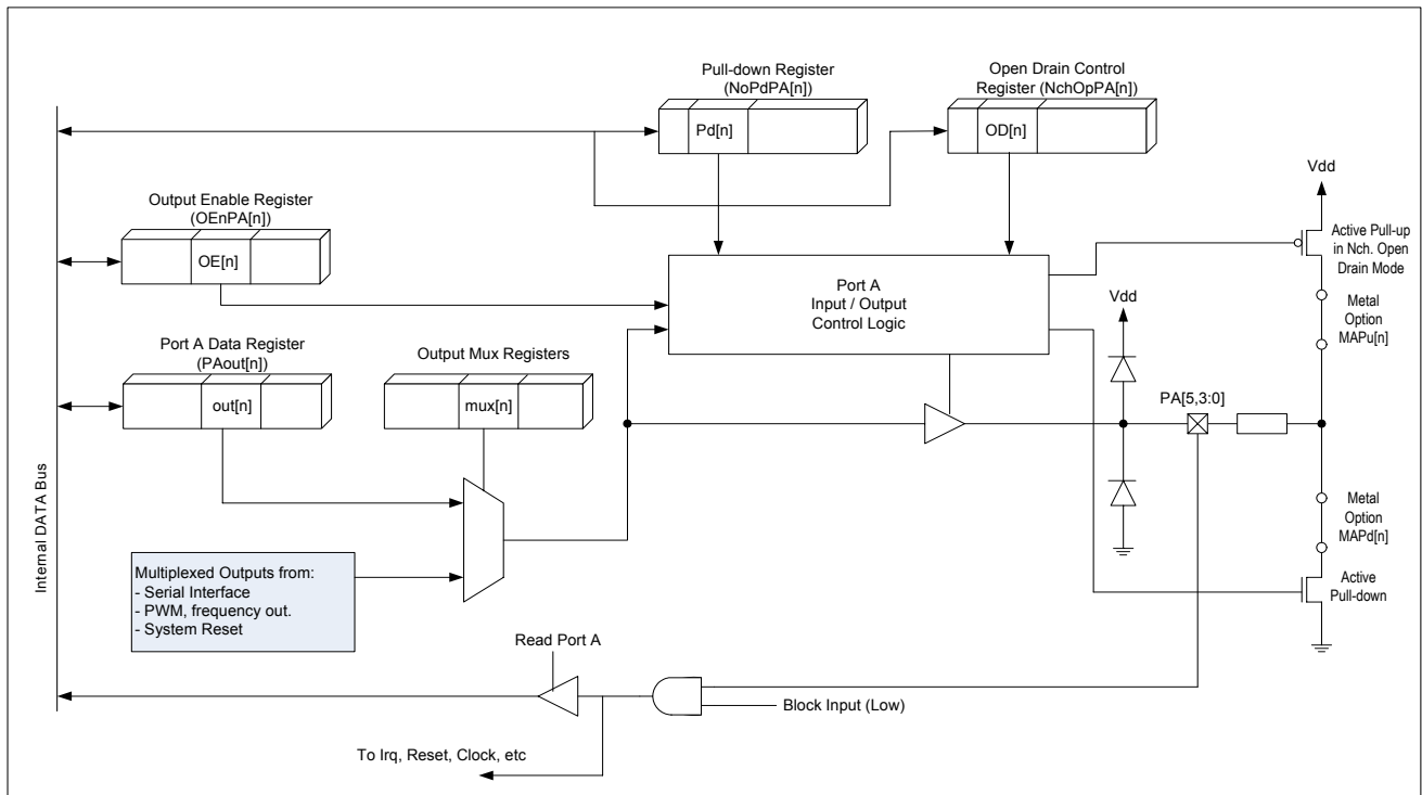
Figure 12. Port A Architecture (Outputs)
