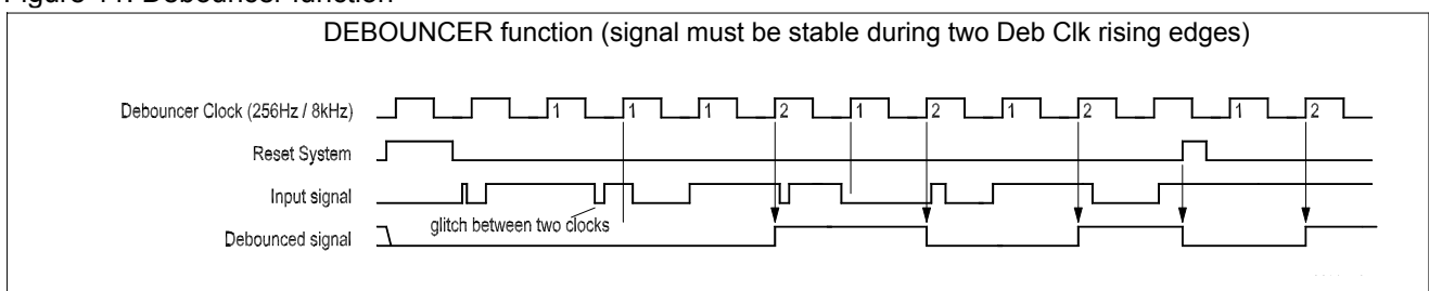
Figure 11. Debouncer function
