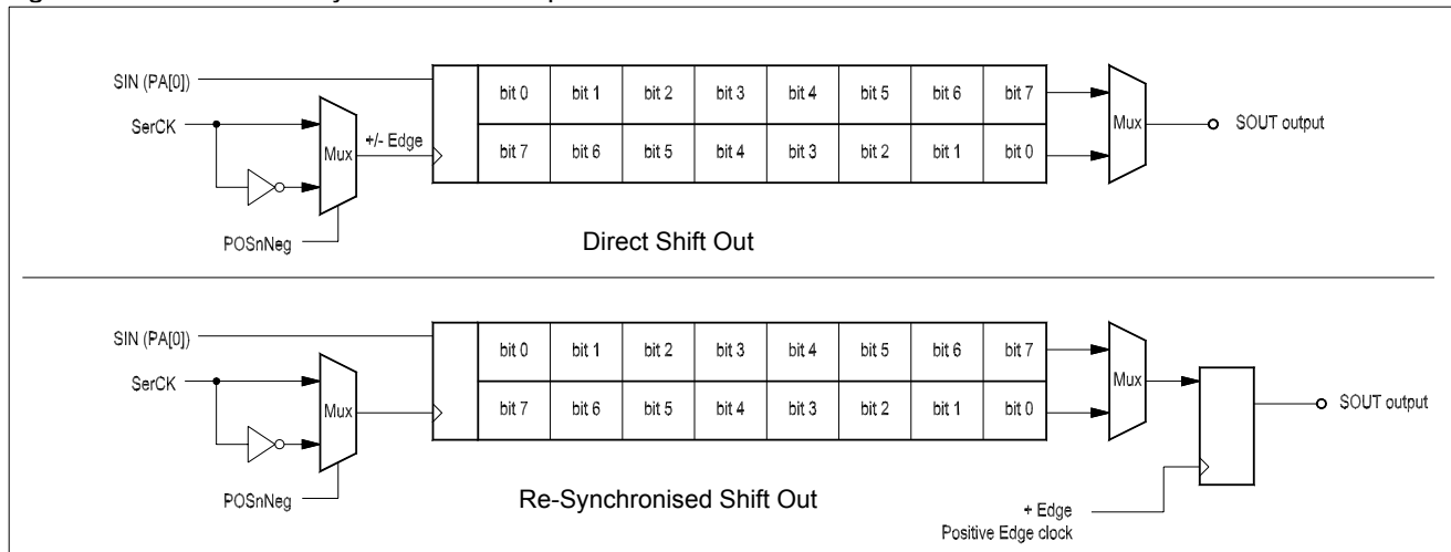
Figure 15. Direct or Re-Synchronized Output
