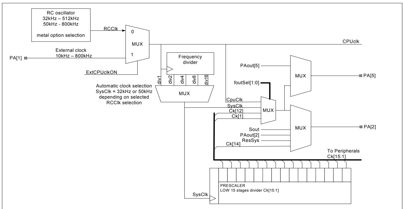
Figure 8. Clock source for CPU or system peripherals
