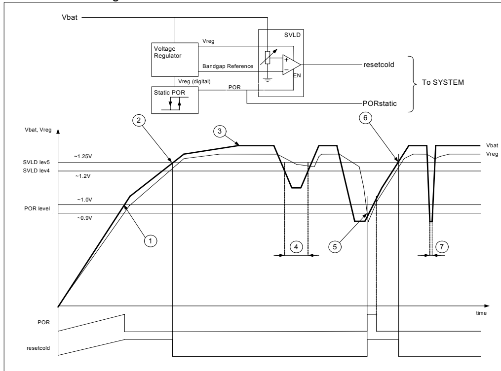
Figure 7. EM6680 resetcold signal as a result of Power-On-Reset and Power-Check
