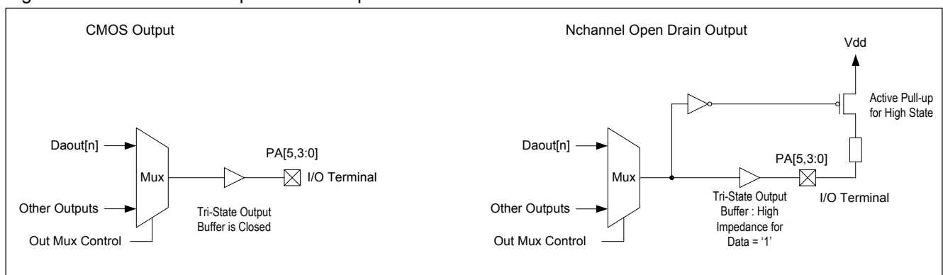
Figure 13. CMOS or Nch. Open Drain Outputs
