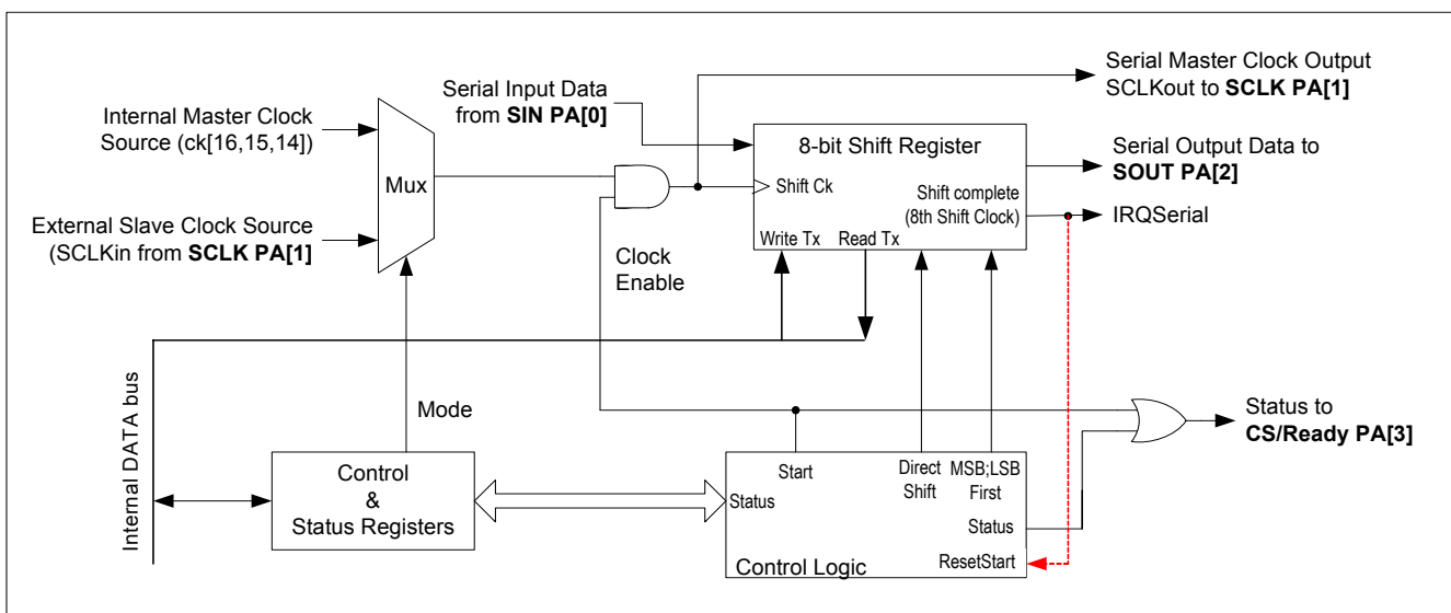
Figure 14. Serial Interface Architecture
