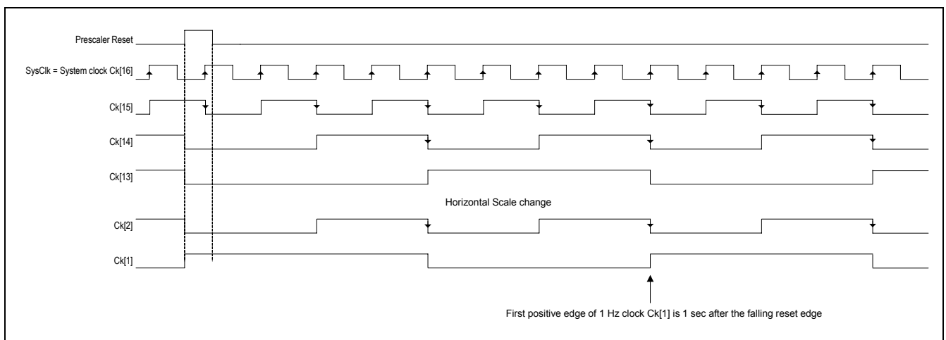
Figure 9. Prescaler Frequency Timing
