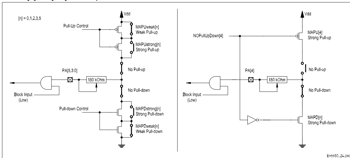
Figure 28. PA[5], PA[3:0] metal option architecture
