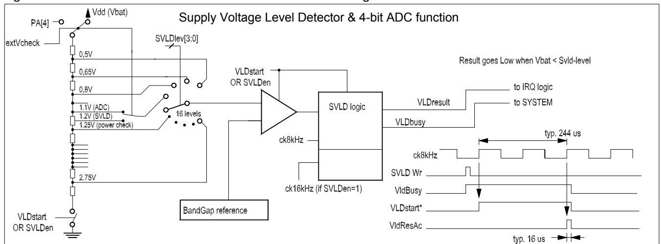
Figure 23. SVLD / 4-bit ADC schematic with controls and timing
