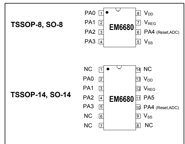
Figure 2. Pin Configuration
