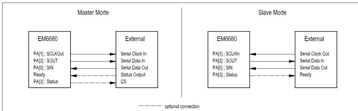
Figure 17. Example of Basic Serial Port Connections
