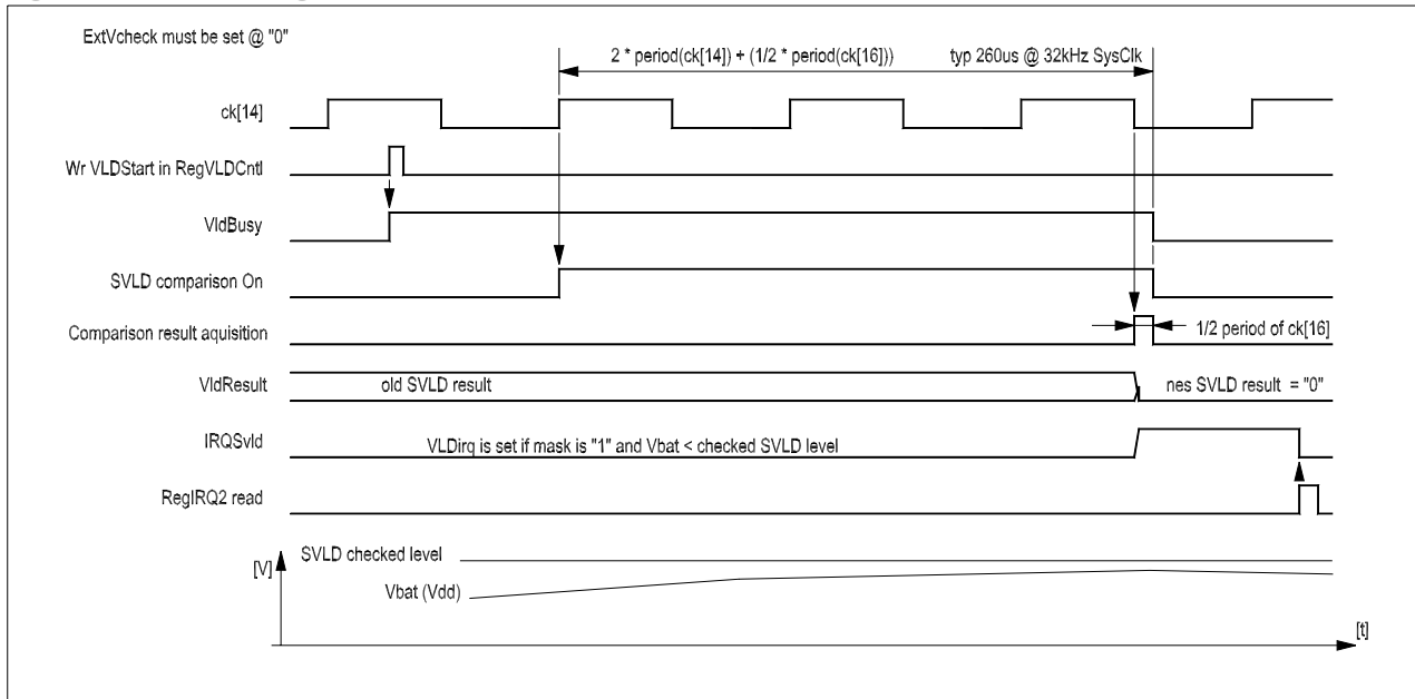
Figure 24. SVLD timing
