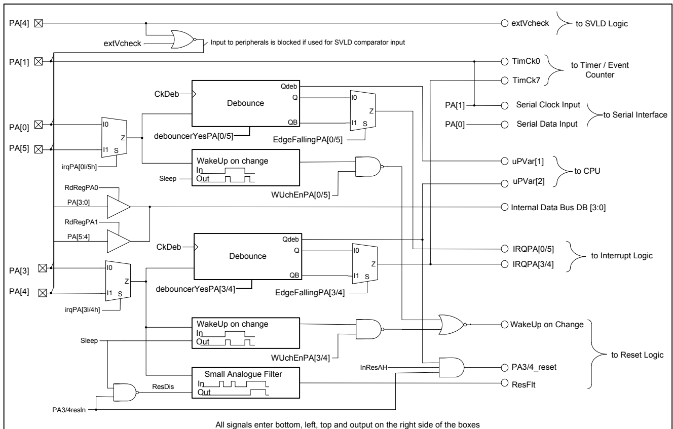
Figure 10. EM6680 Multiplexed Inputs diagram
