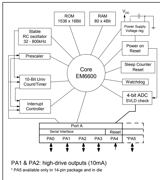
Figure 1. Architecture
