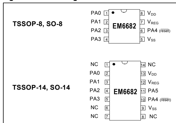
Figure 2. Pin Configuration
