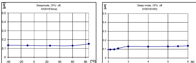
Figure 42. Sleep mode
