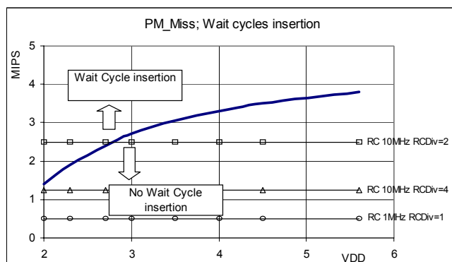
Figure 5. Wait insertion versus Power supply ( V_2 voltage)
