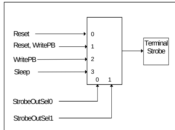
Figure 33 . Strobe Output
