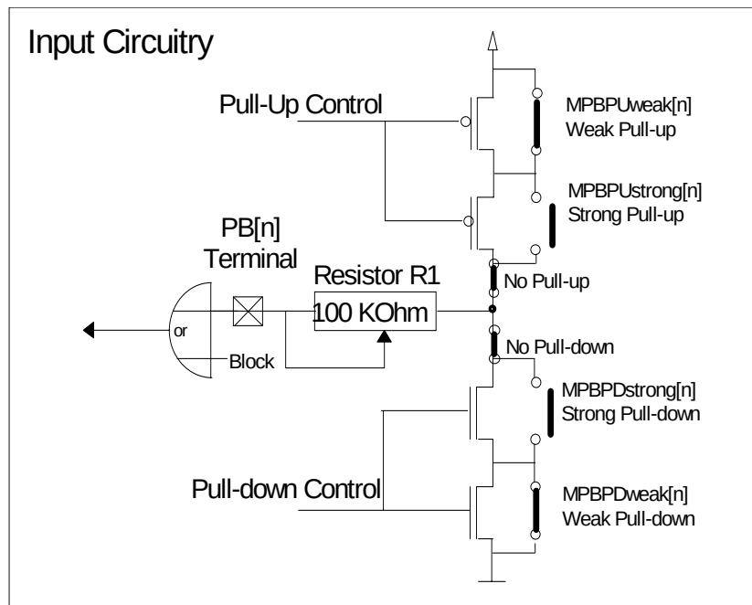
Figure 39. Port B Pull Options
