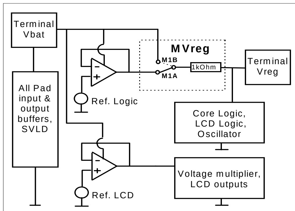
Figure 5. Internal Power Supply
