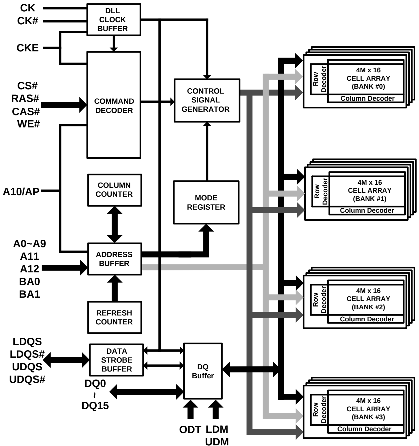
Figure 2. Block Diagram
