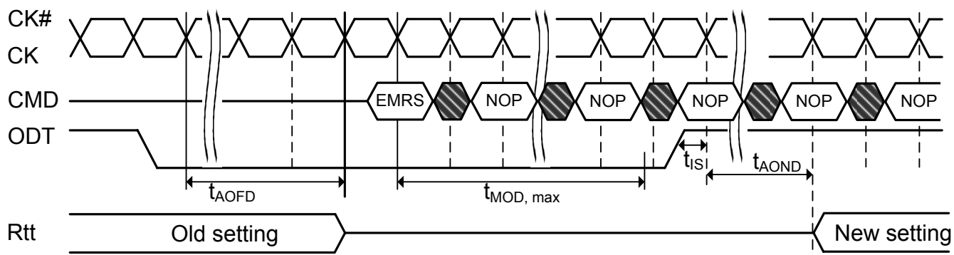
Figure 11. ODT update delay timing- t_{MOD} , as measured from outside
