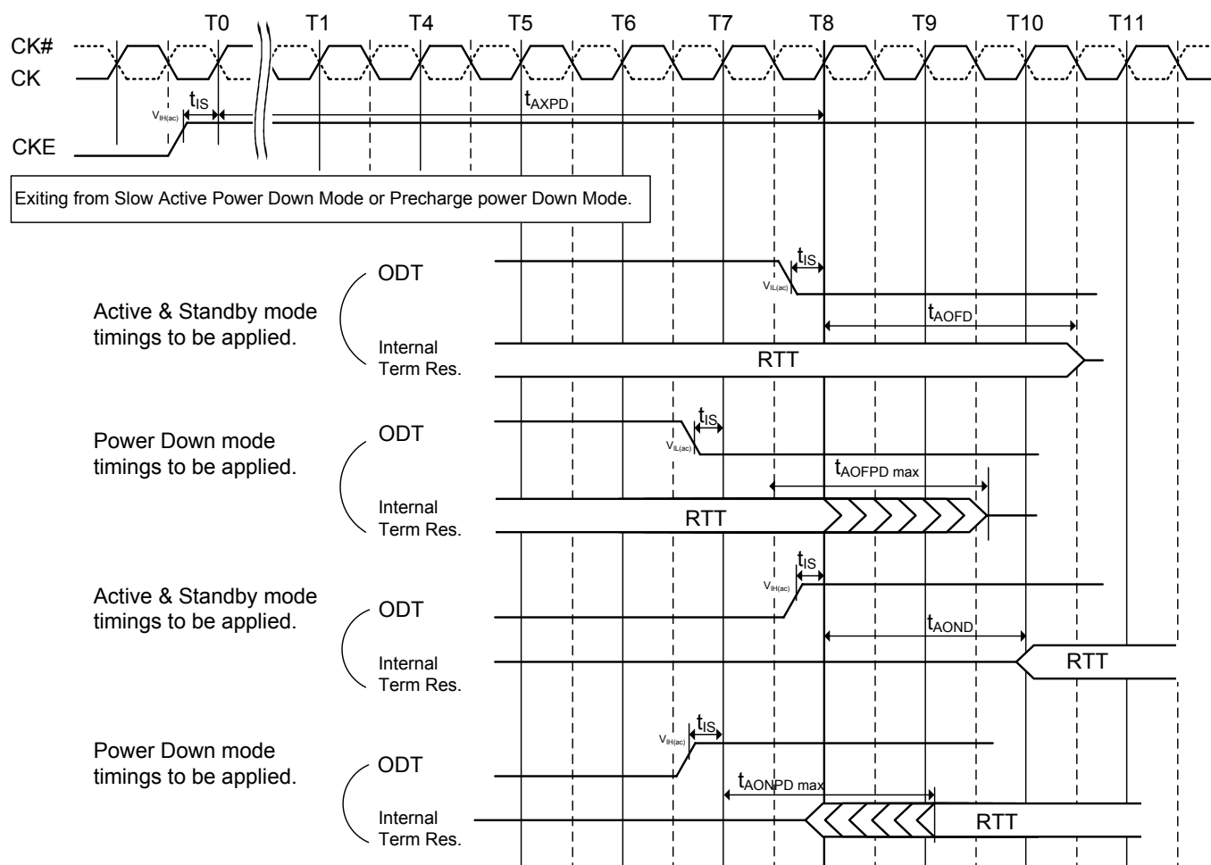
Figure 16.ODT timing mode switch at exit power-down mode
