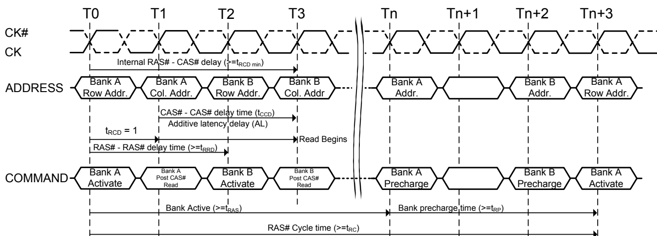
Figure 17. Bank activate command cycle ( t_{\text{RCD}}=3 , \text{AL}=2 , t_{\text{RP}}=3 , t_{\text{RRD}}=2 , t_{\text{CCD}}=2 )
