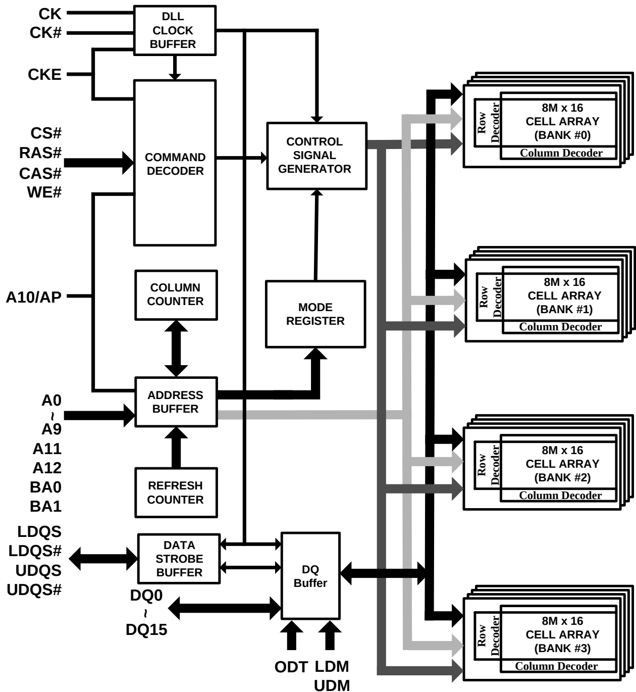
Figure 2. Block Diagram
