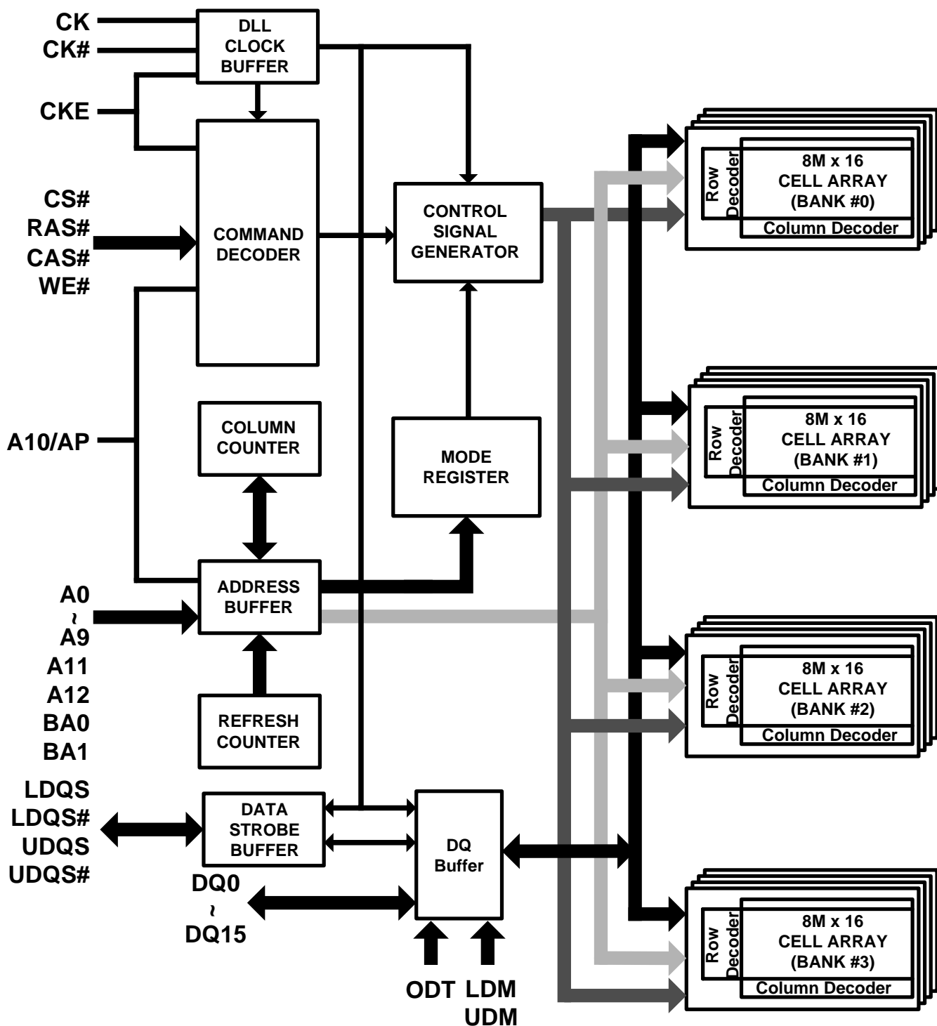
Figure 2. Block Diagram
