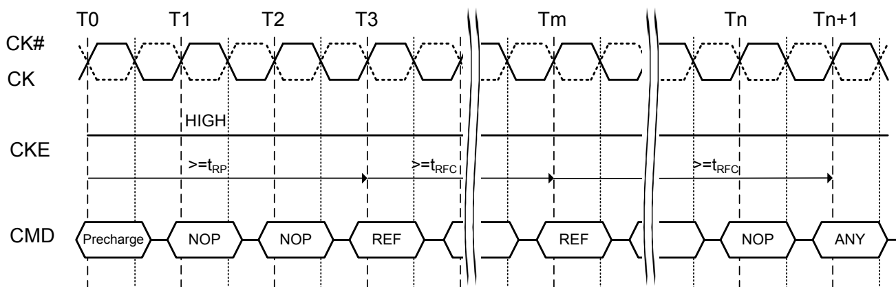
Figure 34. Refresh command
