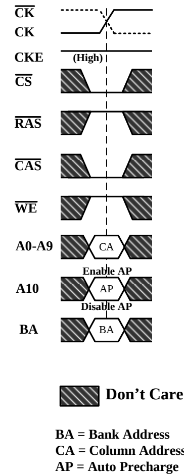
Figure 12. Read Command
