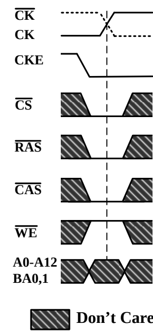
Figure 34. Self Refresh Command
