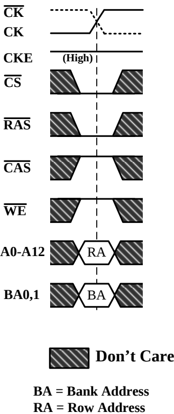
Figure 10. Active Command
