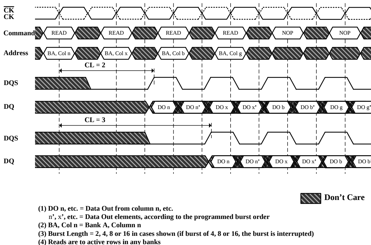
Figure 17. Random Read Bursts
