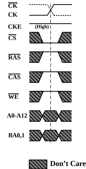
Figure 7. NOP Command
