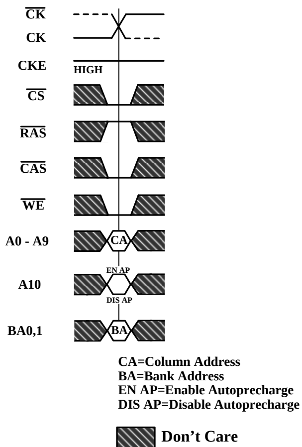
Figure 14. Write Command
