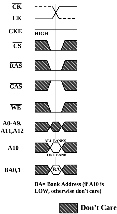
Figure 27. Precharge Command
