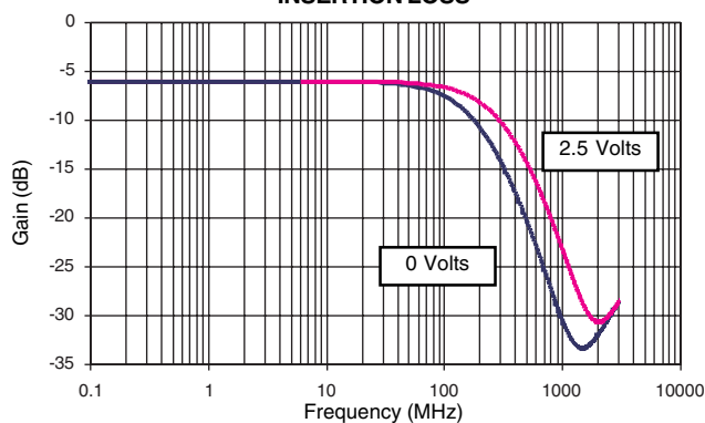
FIGURE 1 INSERTION LOSS
