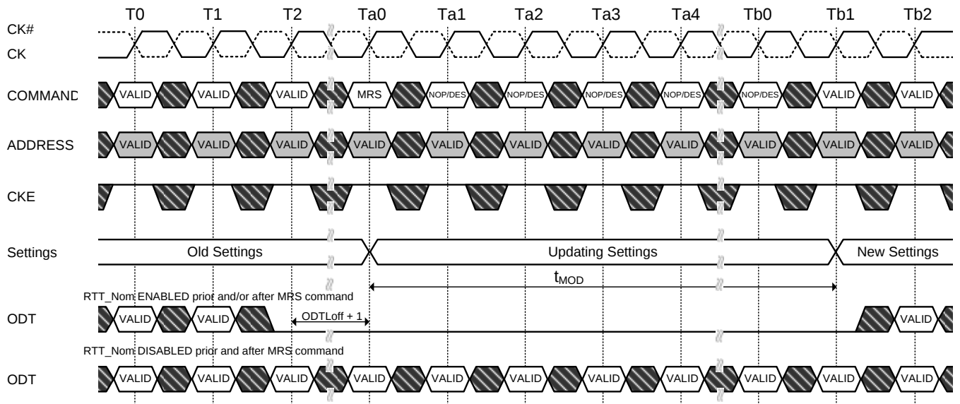
Figure 7. tMOD timing
