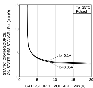
Fig.4 Static Drain-Source On-State Resistance vs. Gate-Source Voltage
