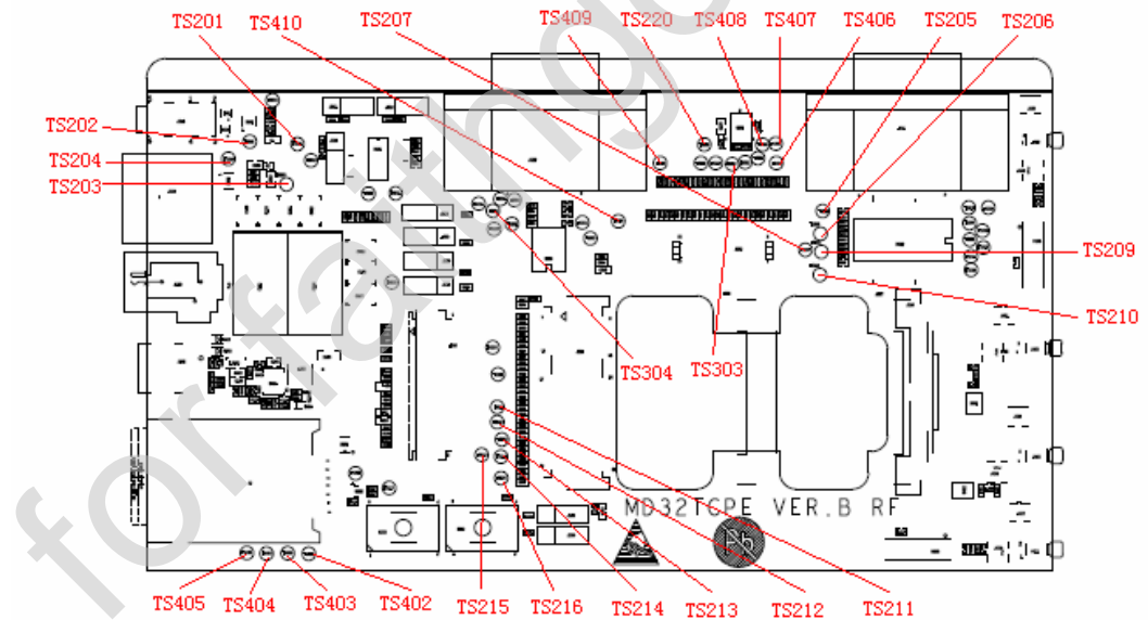
Figure 5-27 Test point position
