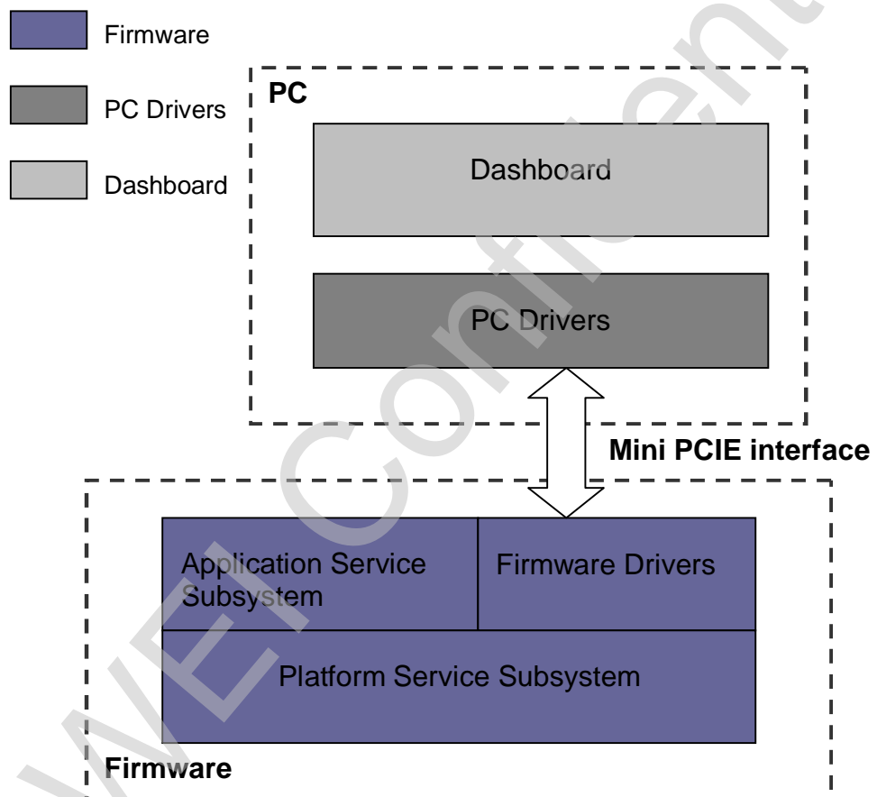
Figure 1-4 Software logic block diagram
