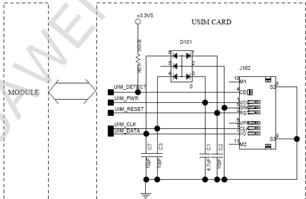
Figure 3-2 USIM interface schematic on PC
