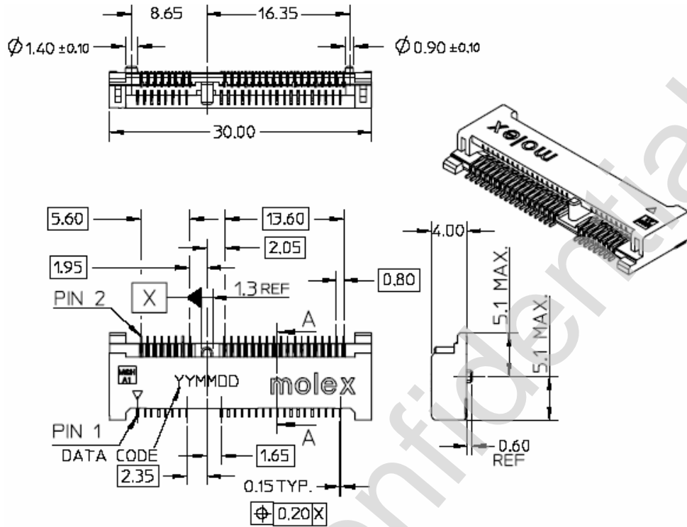
Figure 2-3 Dimensions of the Mini PCI Express connector
