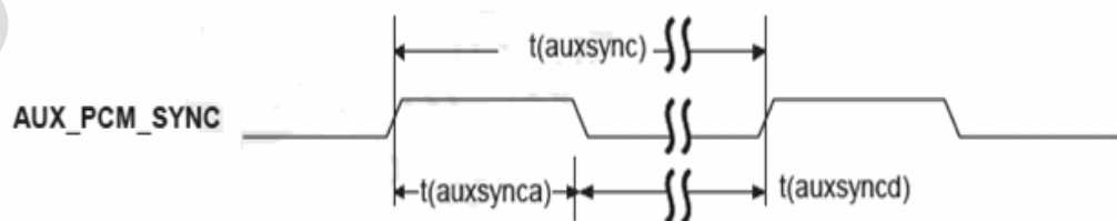
Figure 3-6 AUX_PCM_SYNC timing
