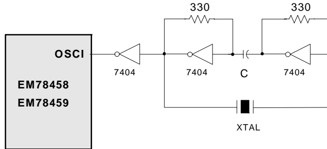
Fig. 20 Circuit for Crystal/Resonator-Series Mode
