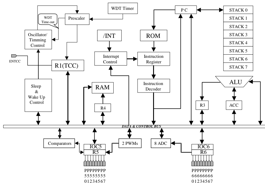
Fig. 2 The Functional Block Diagram of EM78458/459
