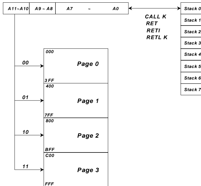
Fig. 3 Program Counter Organization
