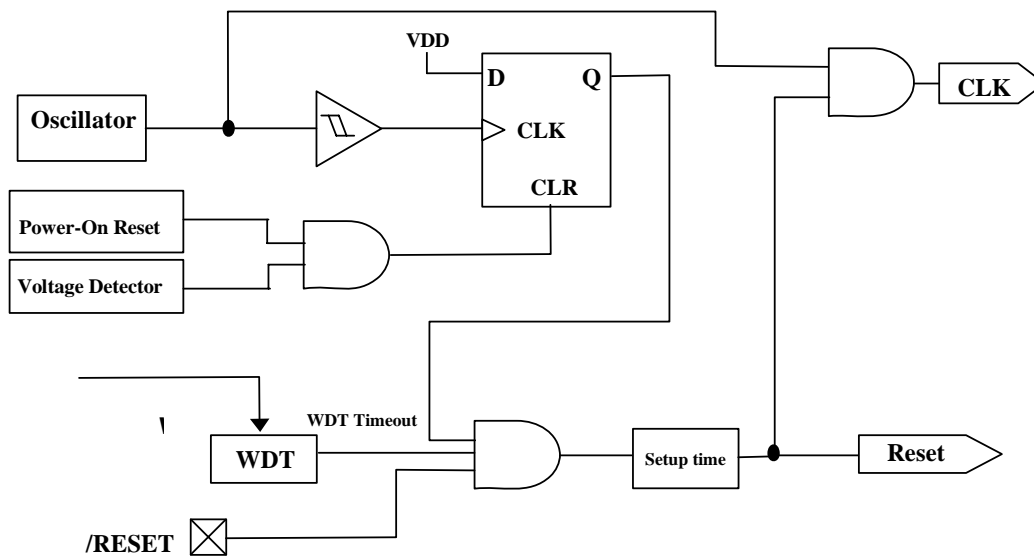
Fig. 10 Block Diagram of Reset of Controller
