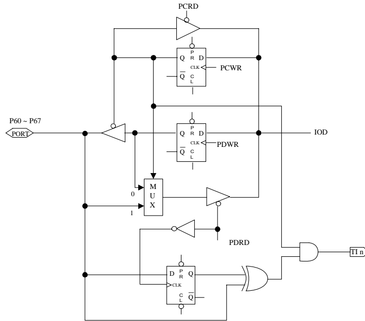
NOTE: Pull-high (down) and Open-drain are not shown in the figure. Fig. 8 The Circuit of I/O Port and I/O Control Register for P60~P67
