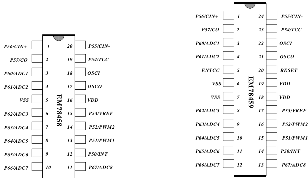
Fig. 1 Pin Assignment
