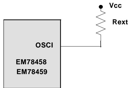
Fig. 23 Circuit for Internal C Oscillator Mode
