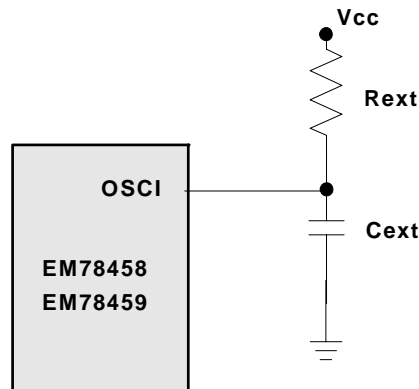
Fig. 22 Circuit for External RC Oscillator Mode
