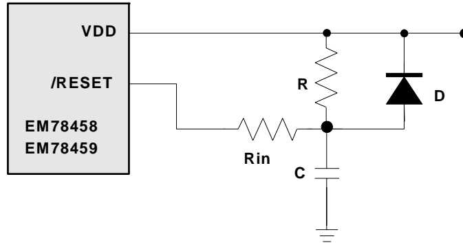
Fig. 24 External Power on Reset Circuit
