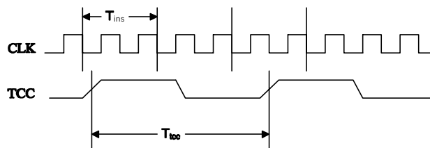
Fig.22 AC timing
