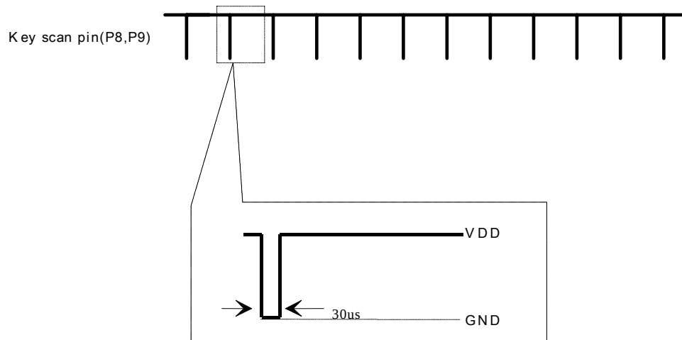
Fig.21 Keyscan Waveform
