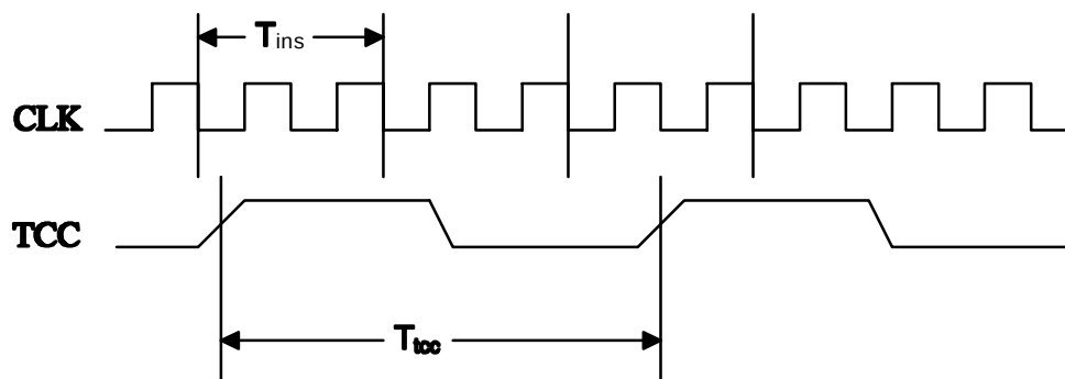
Fig. 30 AC Timing
