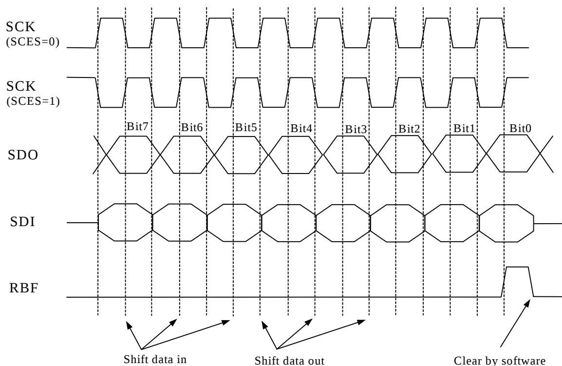
Fig. 14 SPI Timing
