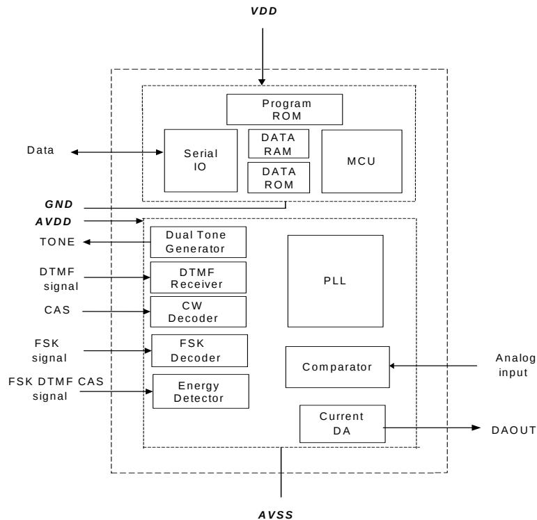
Fig. 2 Block Diagram 1
