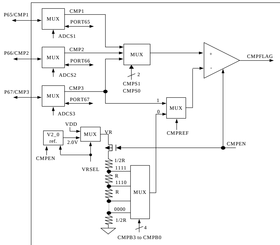
Fig. 19 Comparator Circuit
