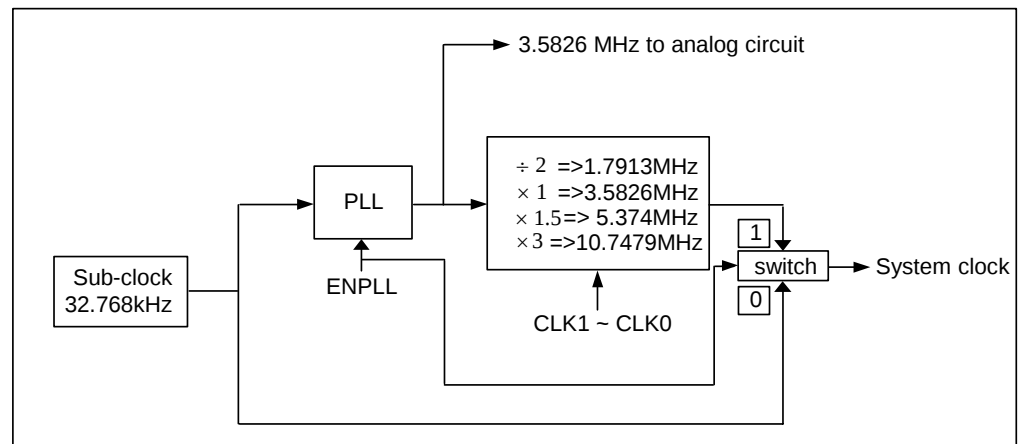
Fig. 18 Relationship between 32.768kHz and PLL
