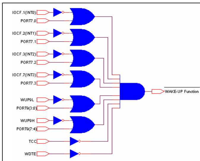
Fig. 6 Wake-up Function and Control Signal
