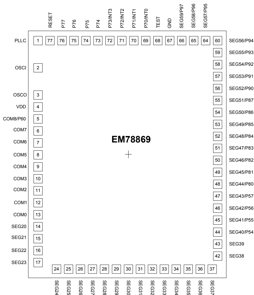
Fig. 1 EM78869 Pin Configuration for Dice Form
