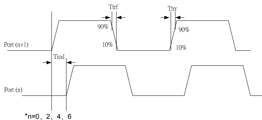
Fig. 15 AC Timing
