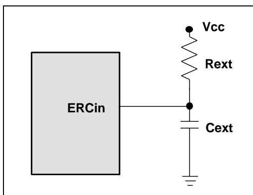
Figure 6-22 External RC Oscillator Mode Circuit
