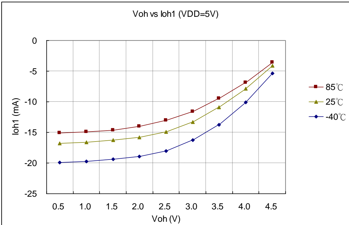
Figure 9-2(a) Voh vs Ioh1, VDD=5V
