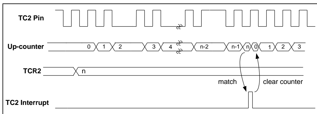
Figure 6-7 Counter Mode Timing Chart
