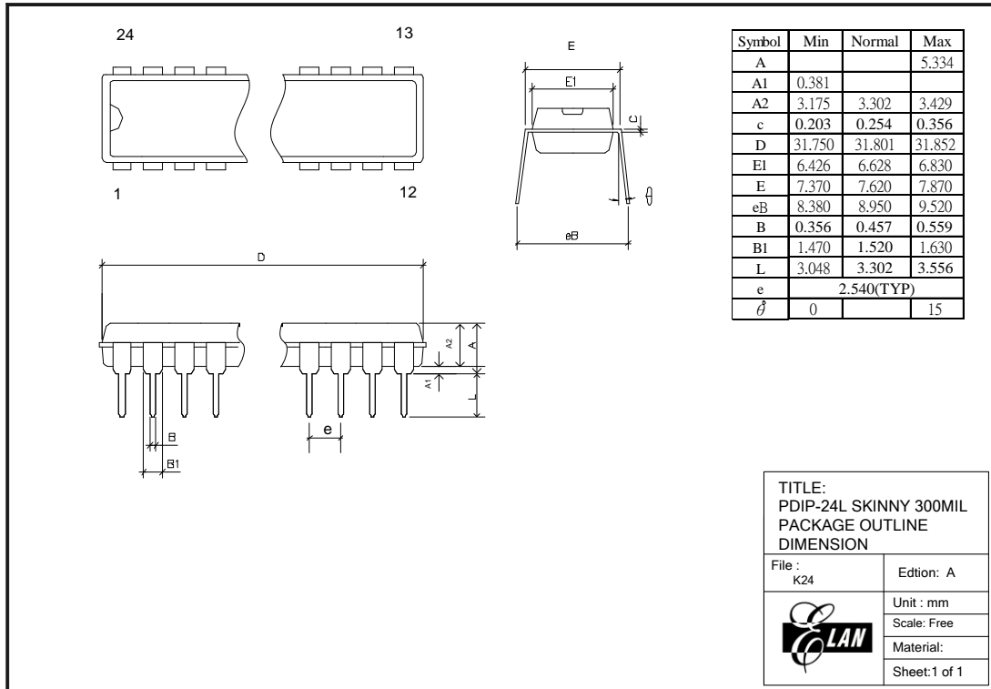
Figure C-1 EM78Fx64N 24-pin Skinny DIP Package Type
