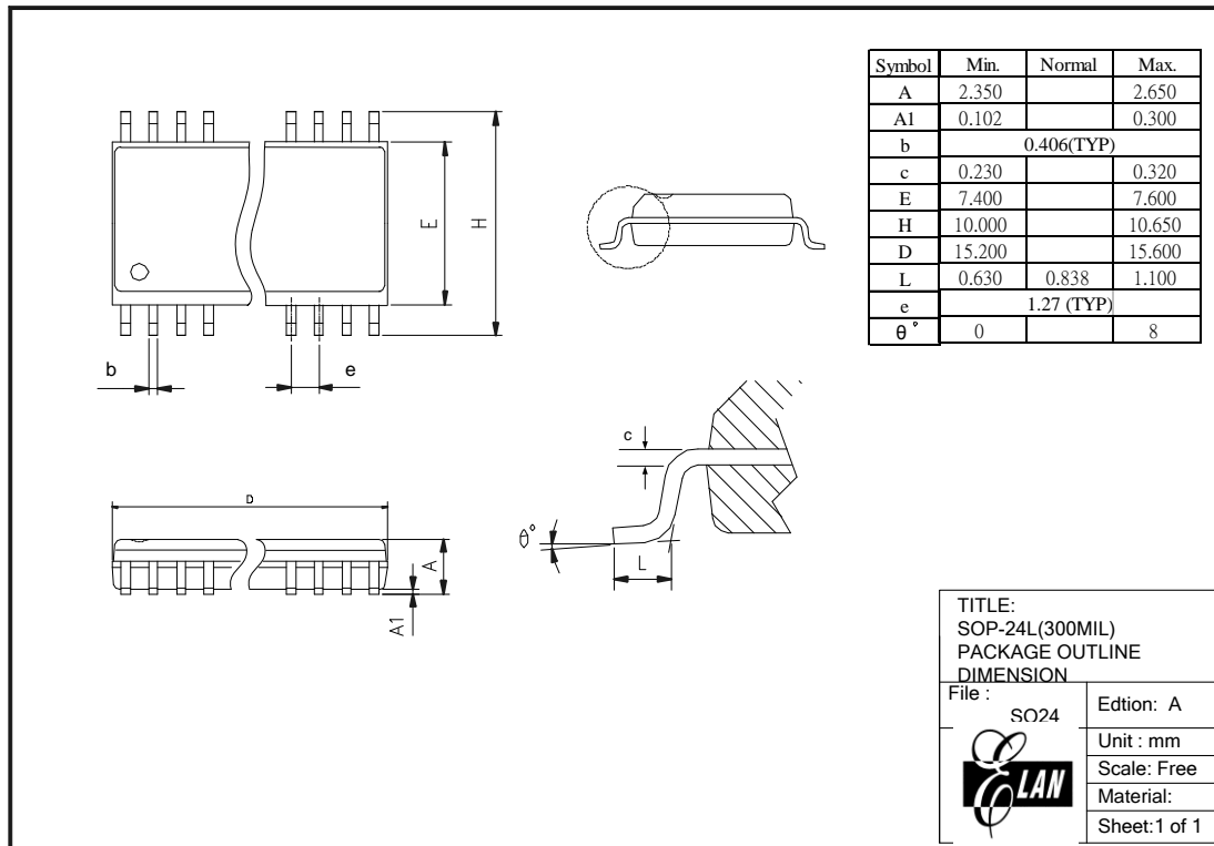
Figure C-2 EM78Fx64N 24-pin SOP Package Type
