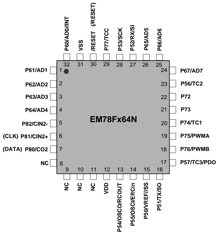
Figure 3-3 32-pin EM78Fx64N
