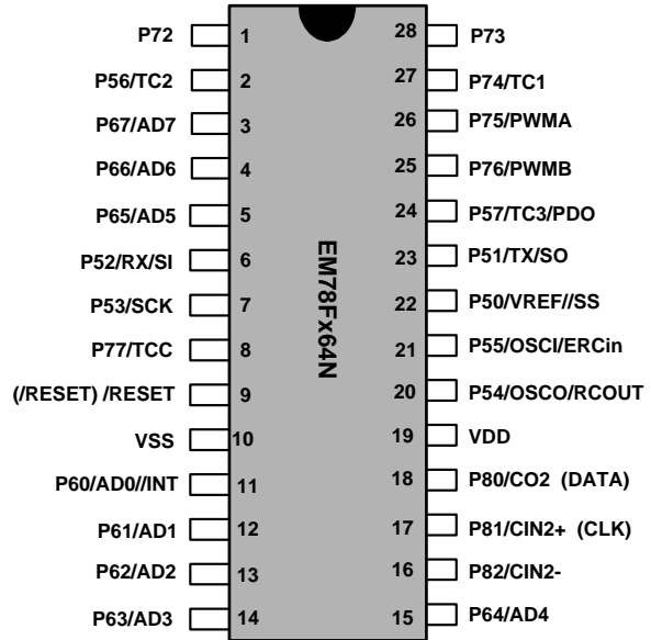
Figure 3-2 28-pin EM78Fx64N
