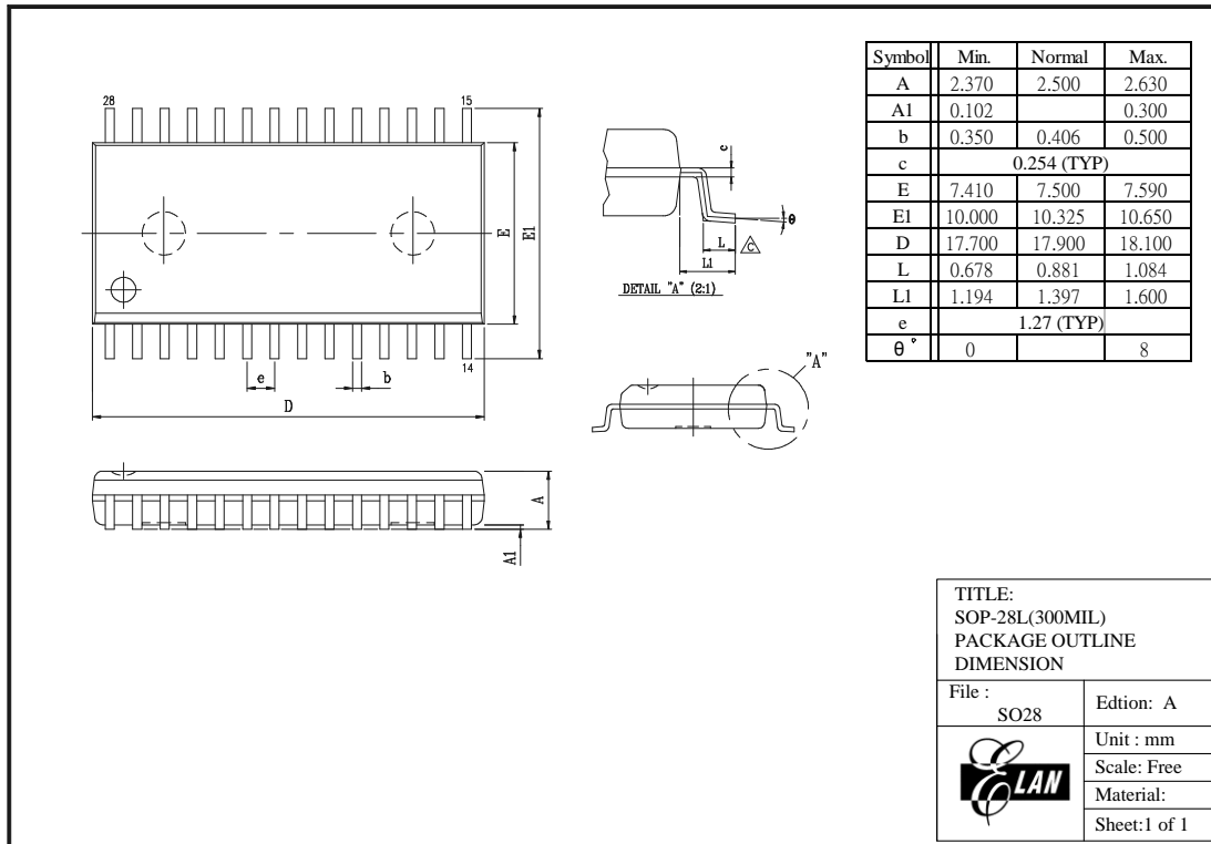
Figure C-4 EM78Fx64N 28-pin SOP Package Type
