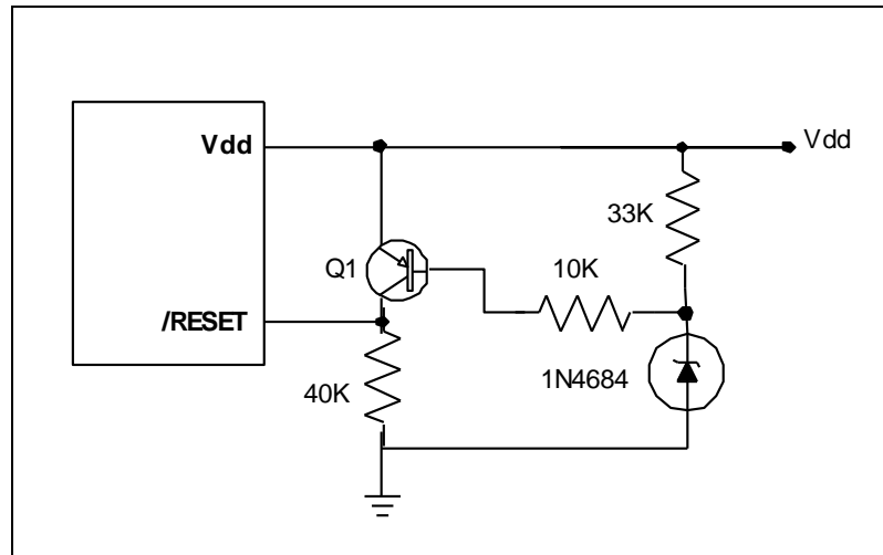
Figure 6-48 Residue Voltage Protection Circuit 1
