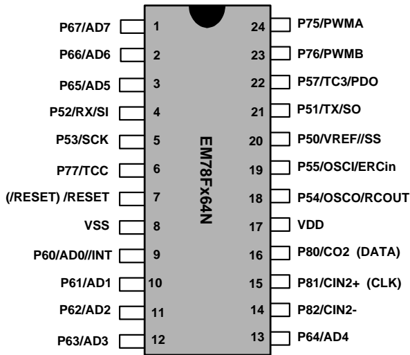
Figure 3-1 24-pin EM78Fx64N
