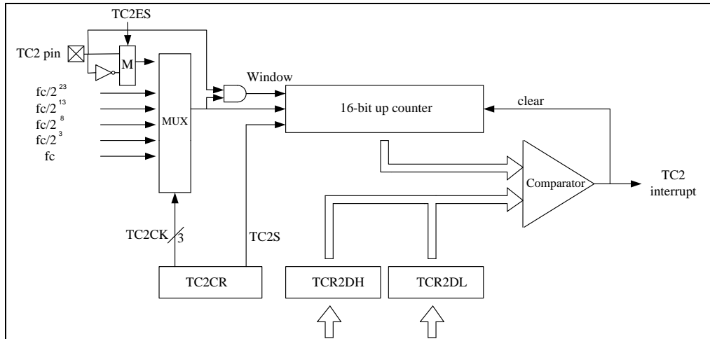
Figure 6-5 Configuration of Timer/Counter 2
