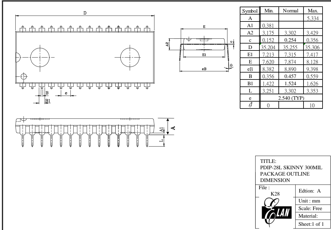
Figure C-3 EM78Fx64N 28-pin Skinny DIP Package Type
