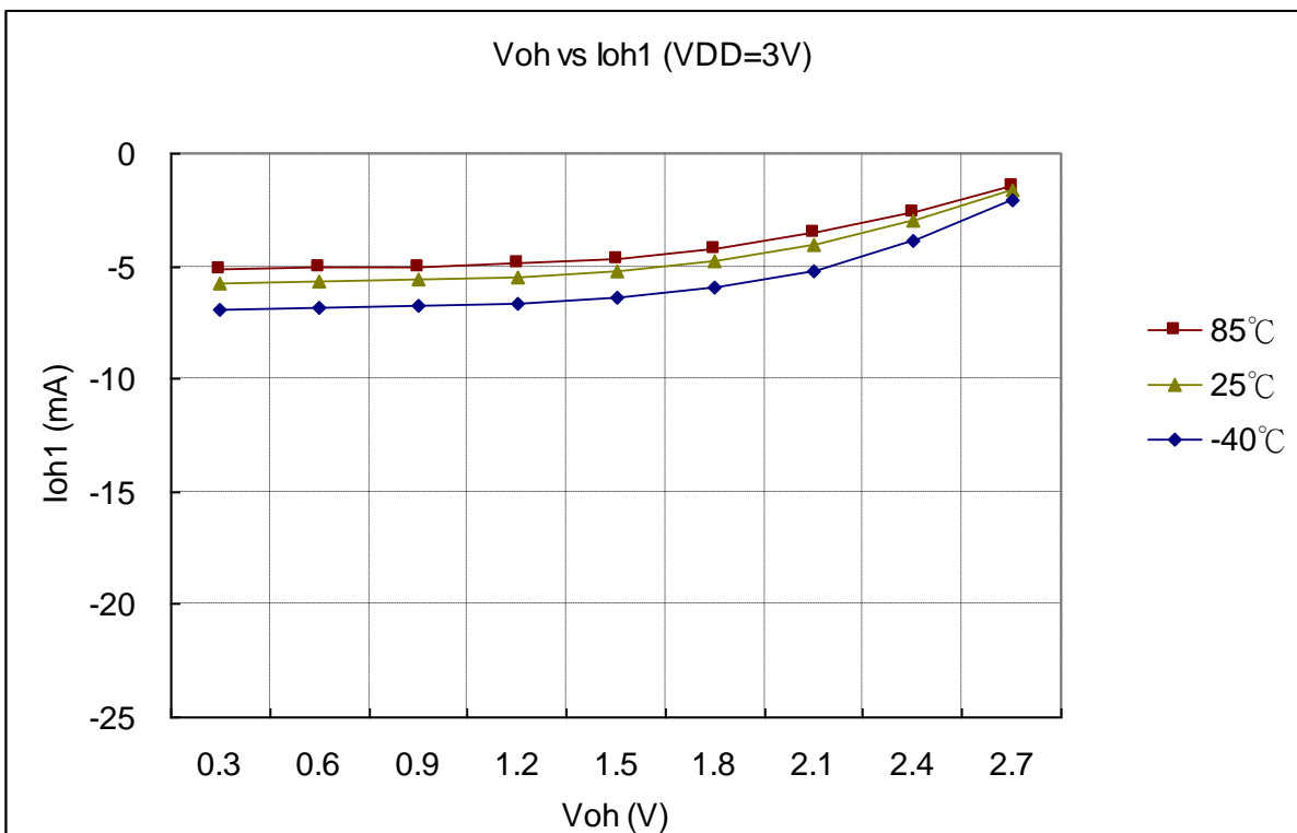
Figure 9-2(b) Voh vs Ioh1, VDD=3V
