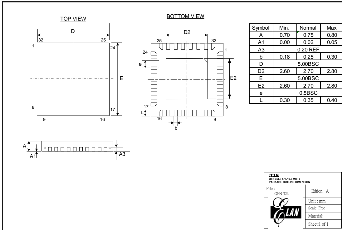
Figure C-5 EM78Fx64N 32-pin QFN Package Type
