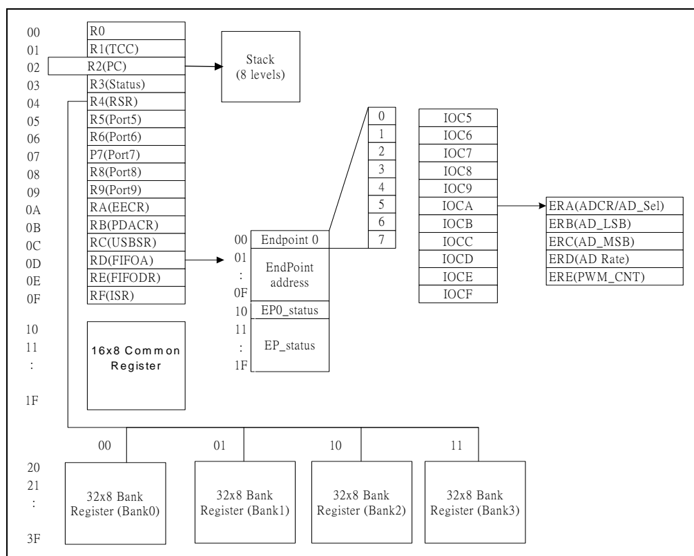
Figure 7-2 Data RAM Organization of EM78M611E
