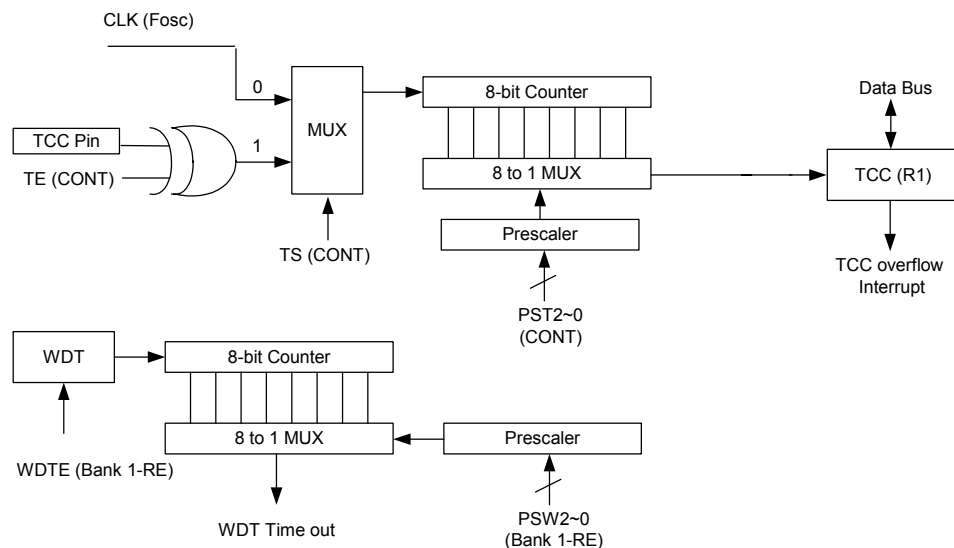
Figure 6-2 TCC and WDT Block Diagram
