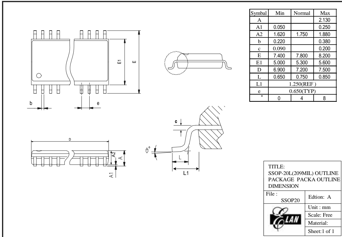
Figure B-3 EM78P210N 20-pin SSOP Package Type
