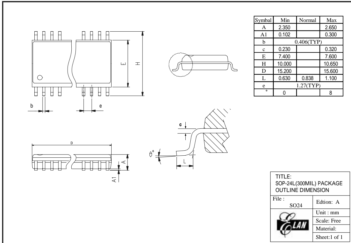
Figure B-5 EM78P210N 24-pin SOP Package Type
