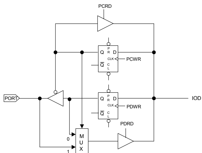
Figure 6-3 I/O Port and I/O Control Register Circuit for Port 5, Port 7 and Port 8
