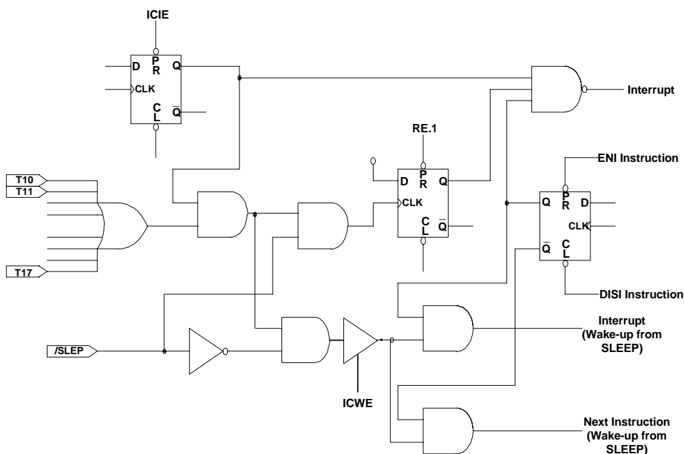
Figure 6-6 Port 6 Block Diagram with Input Change Interrupt/Wake-up
