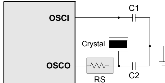
Figure 6-13 Crystal/Resonator Circuit
