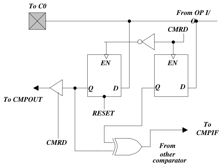
Figure 6-11 Comparator Output Configuration
