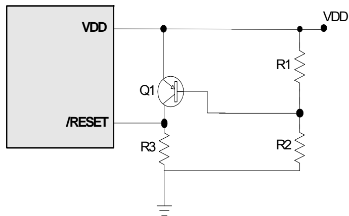
Figure 6-17 Residual Voltage Protection Circuit 2
