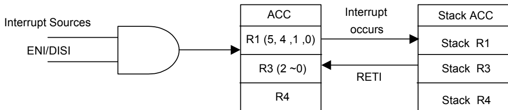
Figure 6-9 Interrupt Backup Diagram
