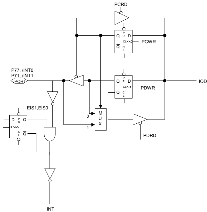
Figure 6-4 I/O Port and I/O Control Register Circuit for P77 (/INT0) and P71 (/INT1)
