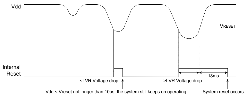
Figure 6-18 LVR Waveform Situation
