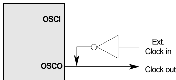
Figure 6-12 External Clock Input Circuit
