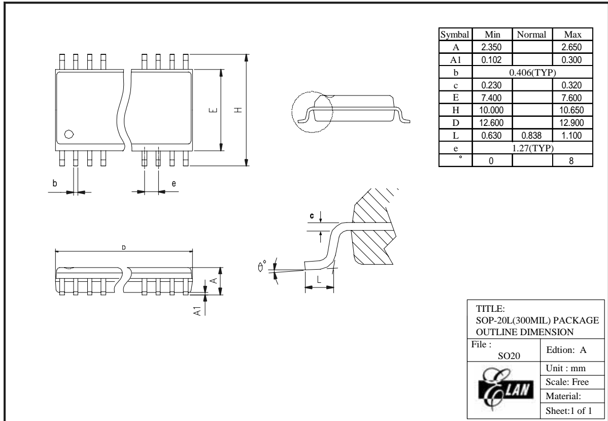
Figure B-2 EM78P210N 20-pin SOP Package Type
