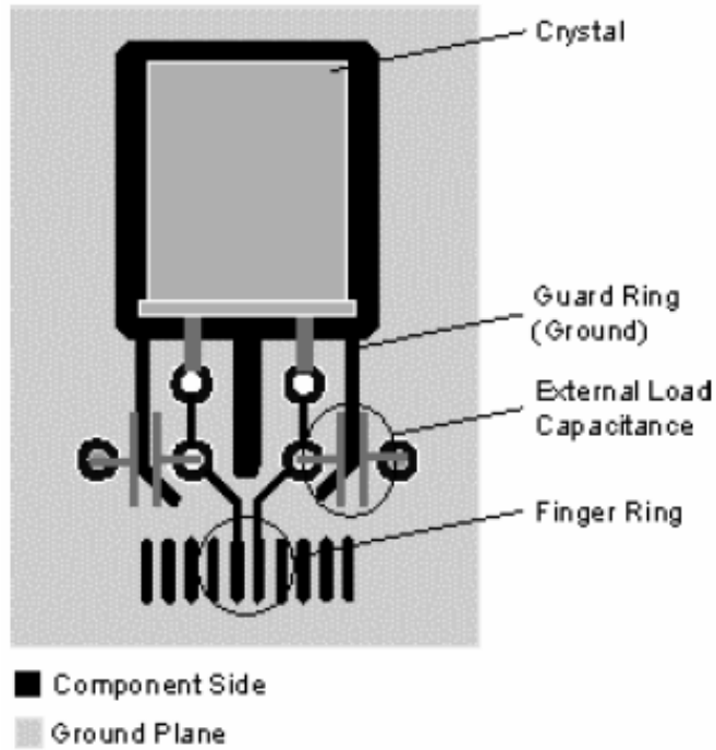
Figure 6-13-1 Parallel Mode Crystal/Resonator Circuit Diagram
