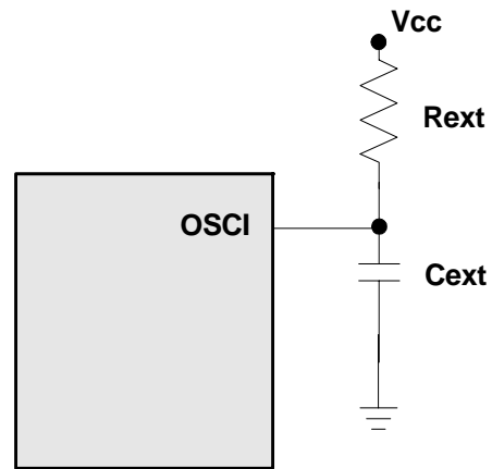
Figure 6-14 External RC Oscillator Mode Circuit
