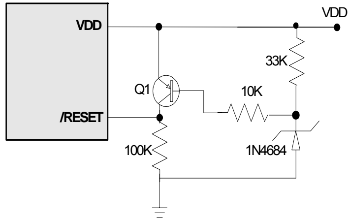
Figure 6-16 Residual Voltage Protection Circuit 1
