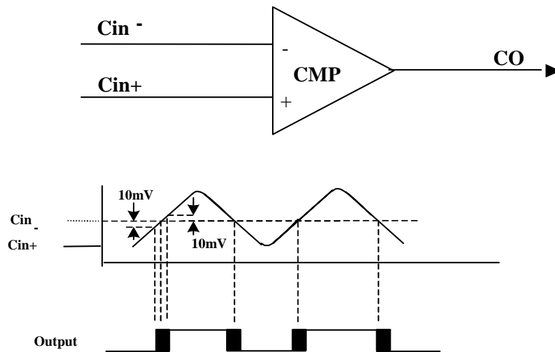
Figure 6-10 Comparator Circuit Diagram & Operating Mode
