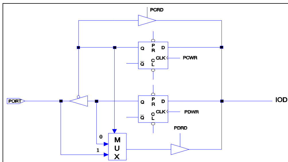
Figure 8-2 Circuit of I/O port and I/O Control Register for Port 5 ~ Port 9
