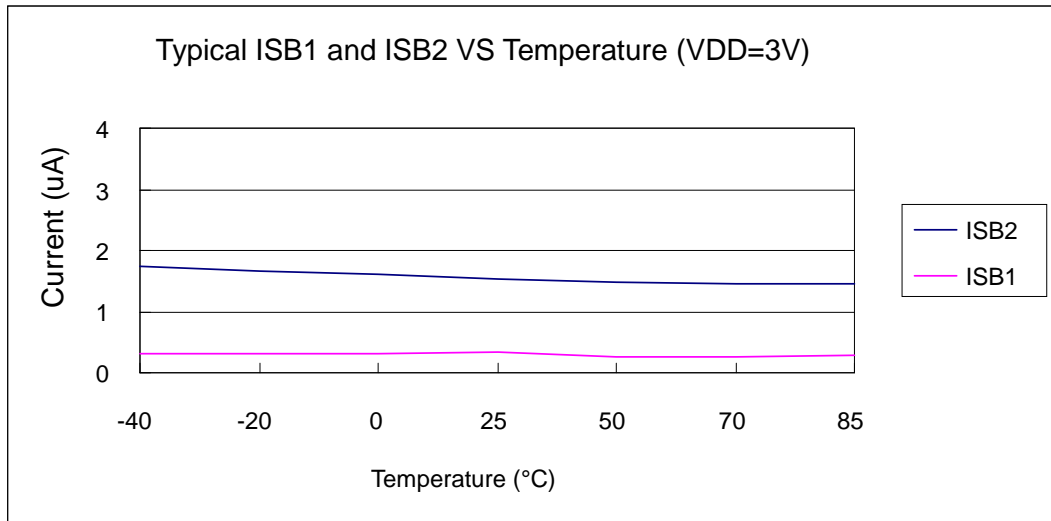
Figure 8-11 Typical Standby Current (VDD=3V) vs. Temperature
