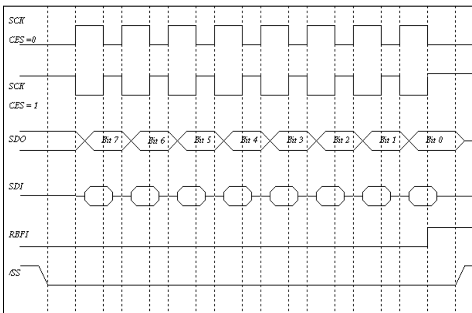
Figure 6-25 SPI Mode with /SS Enabled
