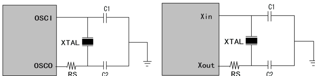
Figure 6-7-1 Circuit for Crystal/Resonator
