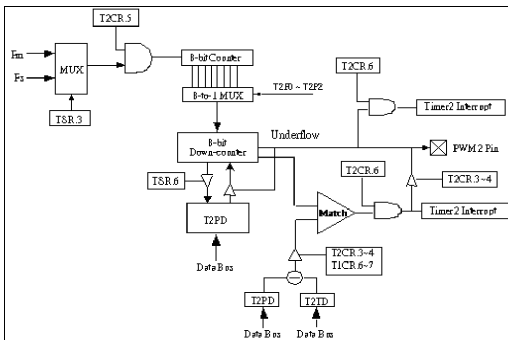
Figure 6-30 Timer 2 Configuration
