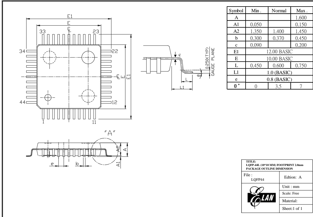
Figure B-4 EM78P520N 44-pin LQFP Package Type
