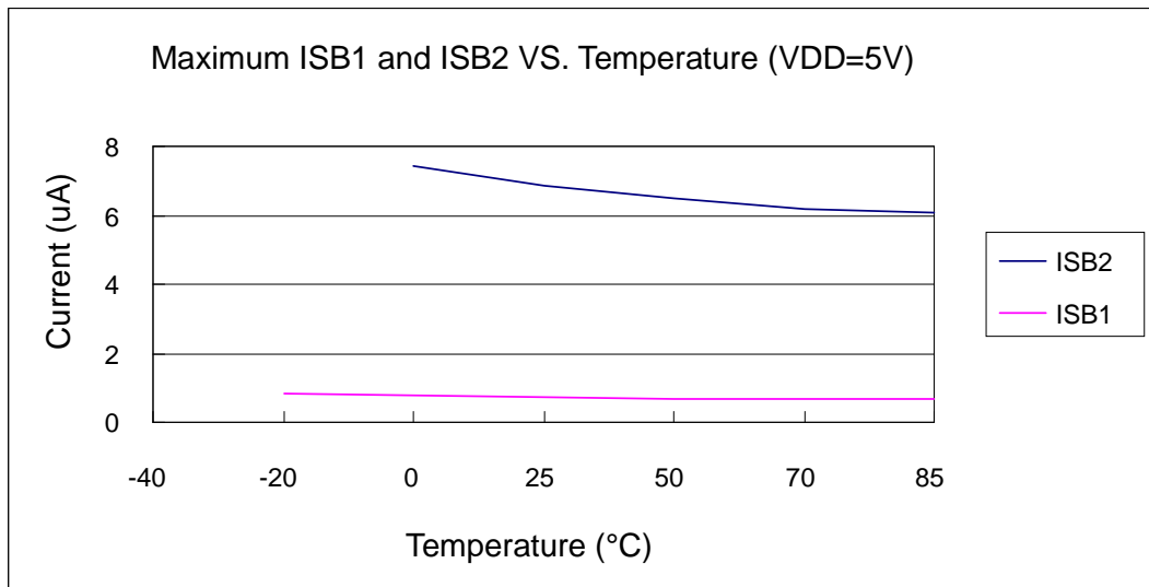
Figure 8-14 Maximum Standby Current (VDD=5V) vs. Temperature
