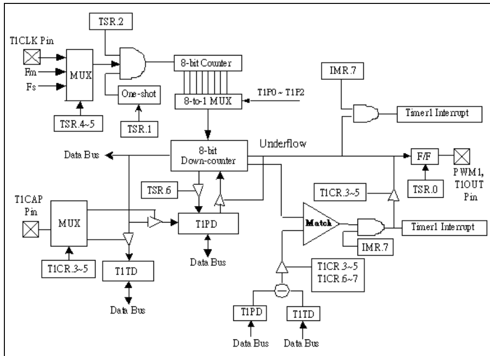
Figure 6-26 Timer/Counter 1 Configuration
