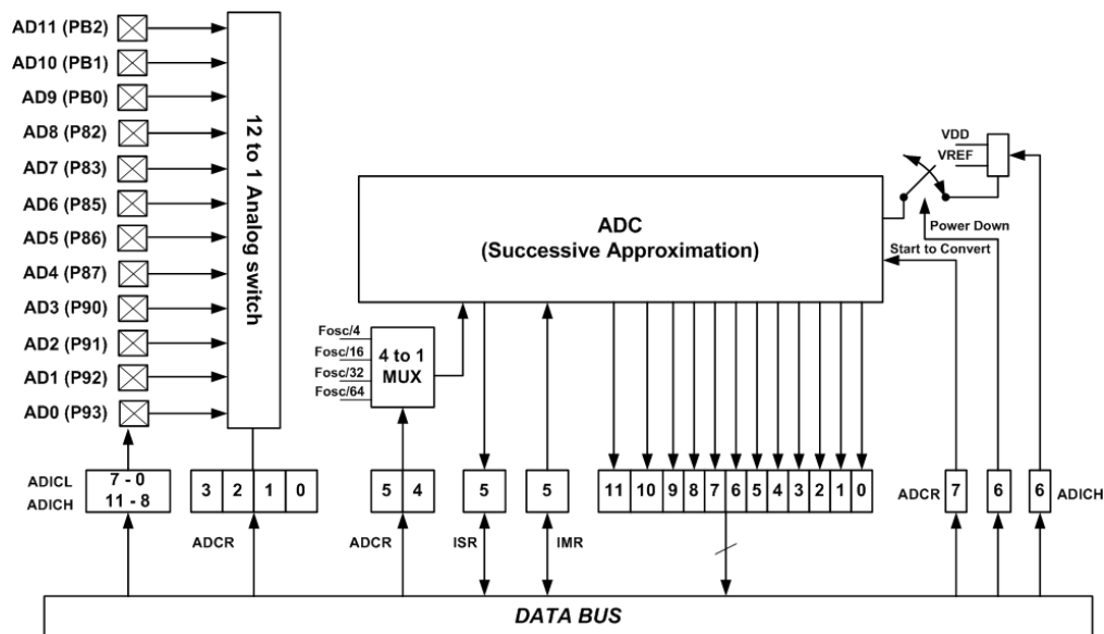
Figure 6-16 AD Converter
