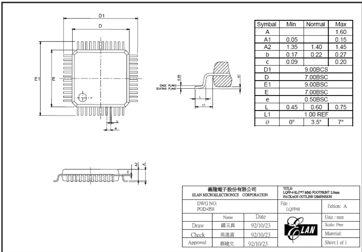
LQFP-48 dimension
