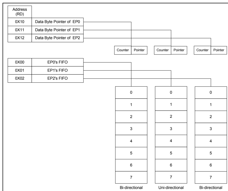
Figure 7-4 EM78P611G USB Application FIFO
