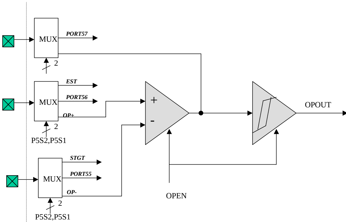
Fig.24 OP structure
