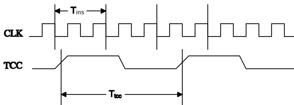
Fig.28 AC timing
