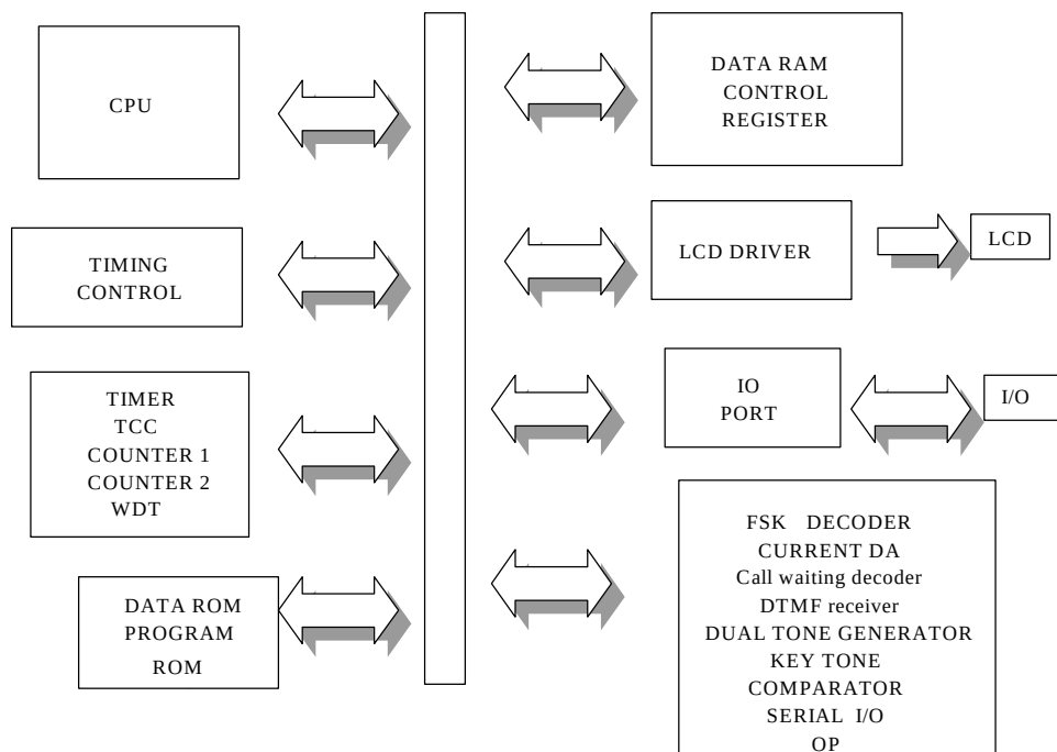
Fig.2 Block diagram1
