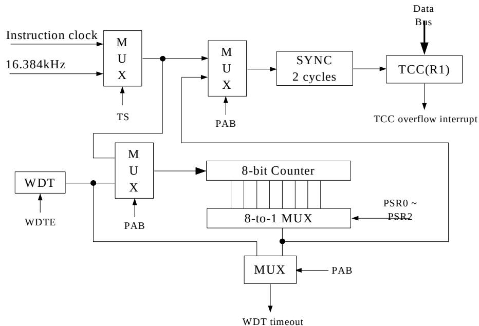
Fig.17 Block diagram of TCC WDT
