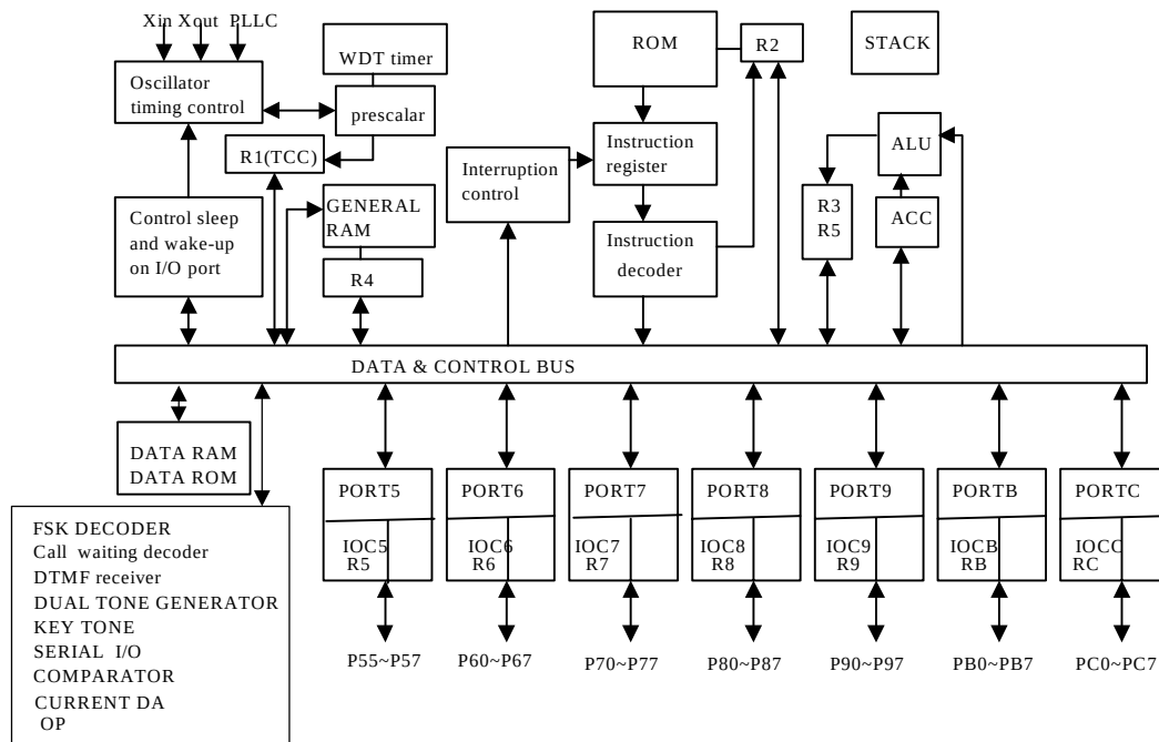
Fig.3 Block diagram2
