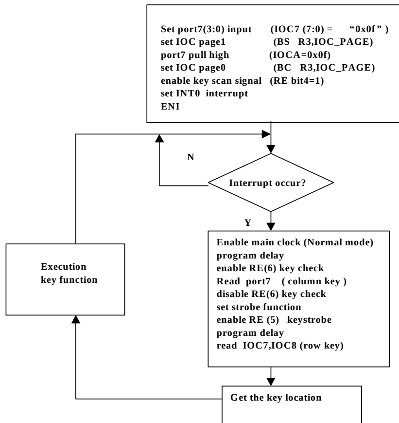
Fig.16 key scan flow by interrupt trigger
