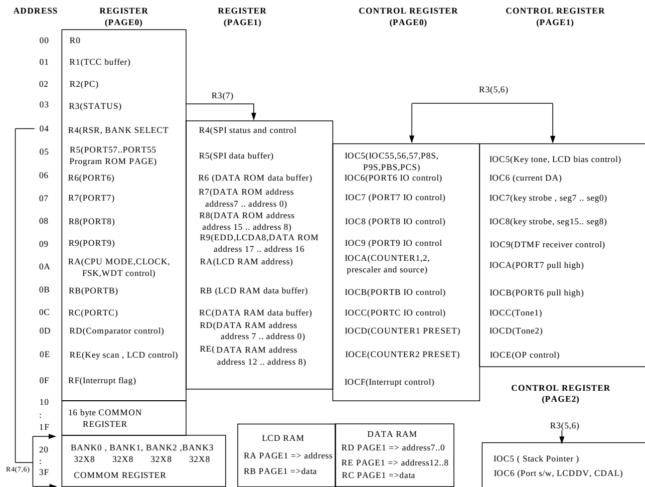
Fig.4 control register configuration
