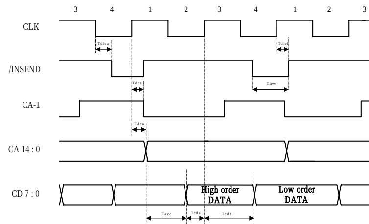
Fig.33 Data ROM access timing
