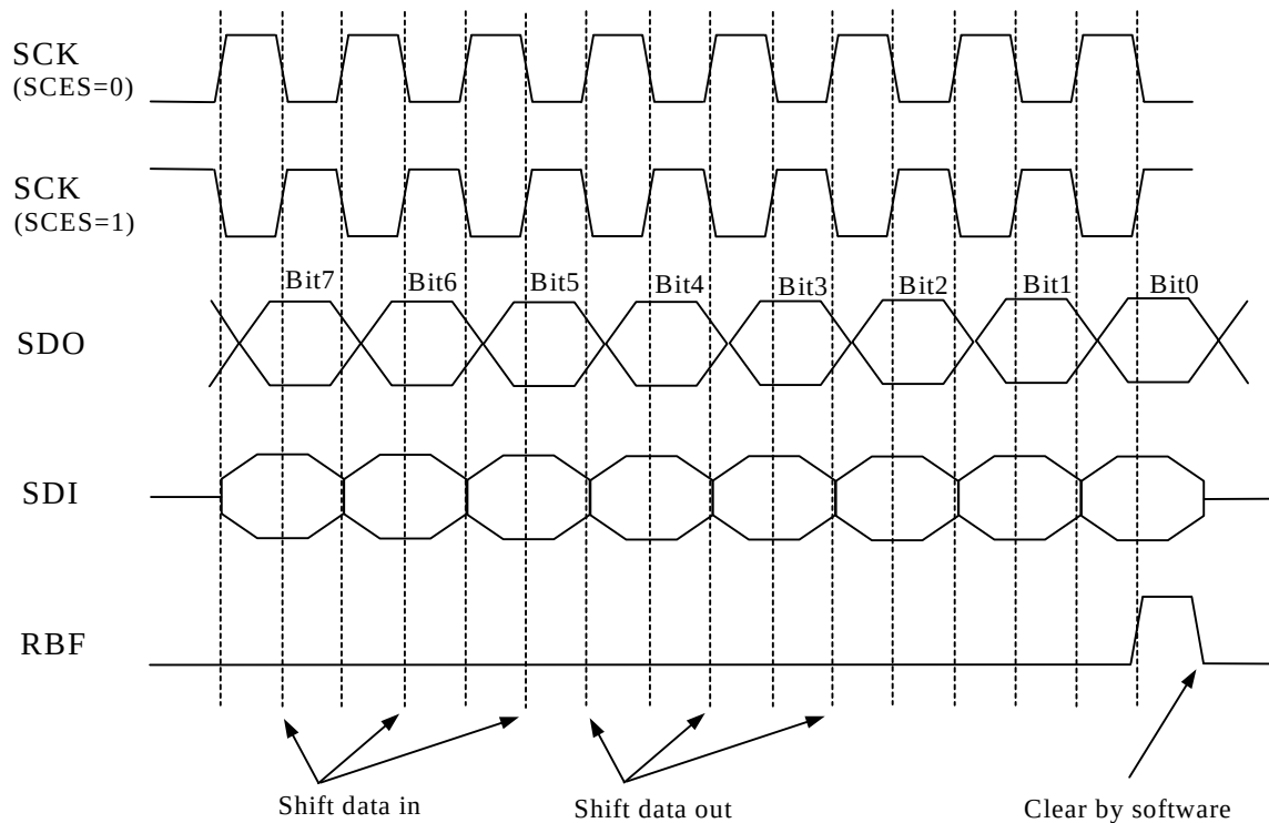
Fig.8 SPI timing
