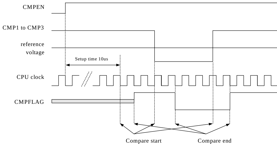
Fig.12 Comparator timing
