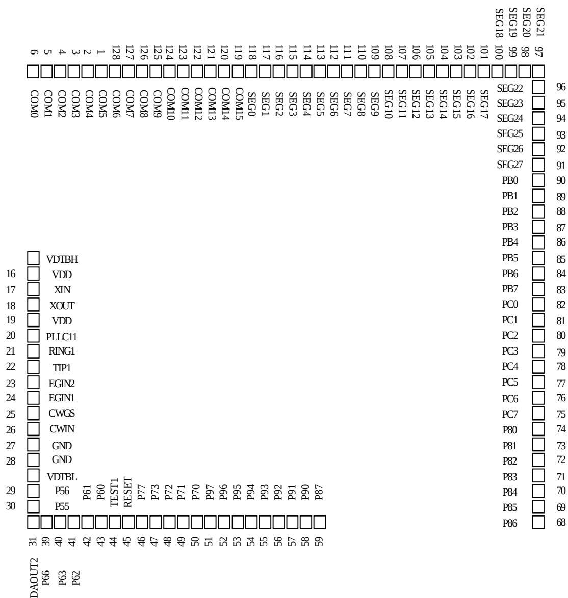
Figure 2-1, Pad assignment (for chip)
