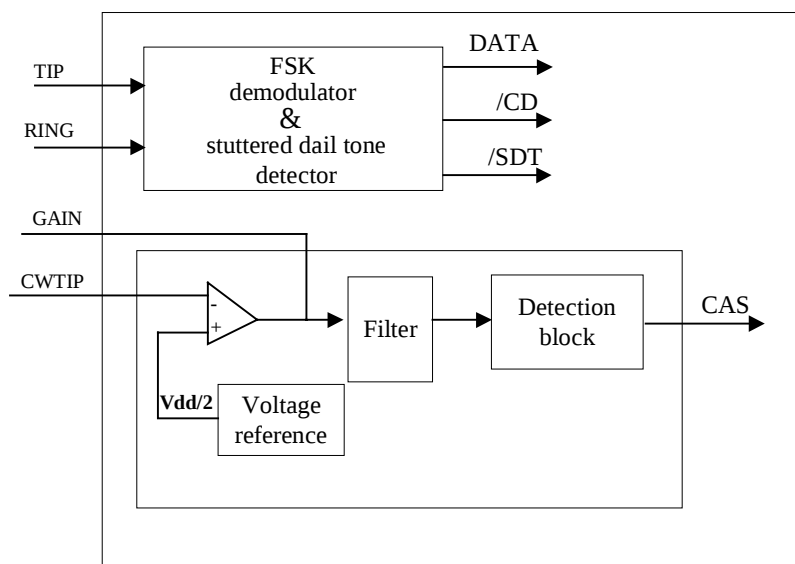
Figure 27, Call Waiting Block Diagram
