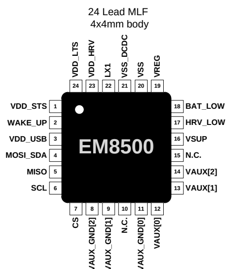
Figure 1-1 QFN24 Package
