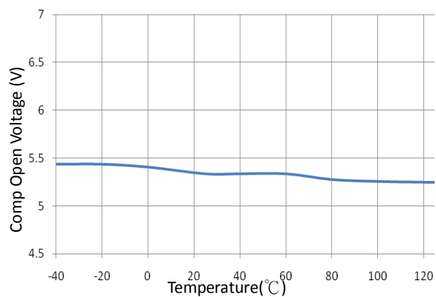
Fig7. Comp Open Voltage vs. Temperature.
