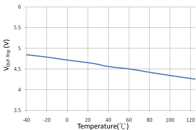
Fig6. V OLP-Trip vs. Temperature.
