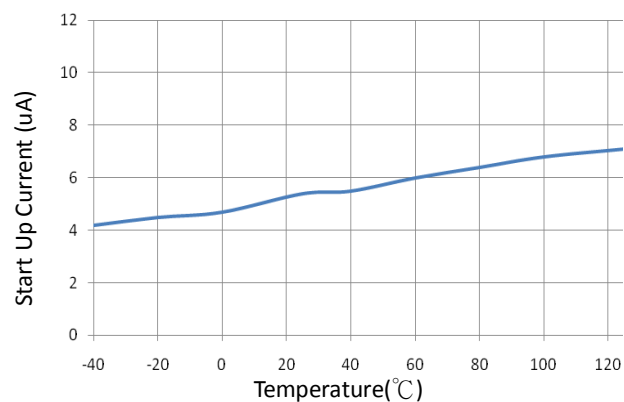
Fig4. Start Up Current vs. Temperature.
