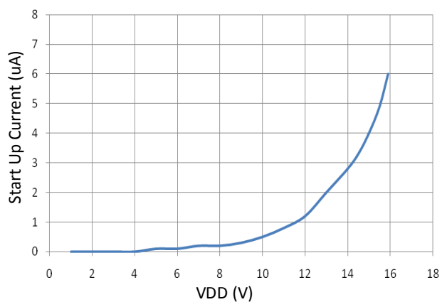
Fig8. Start Up Current vs. VDD
