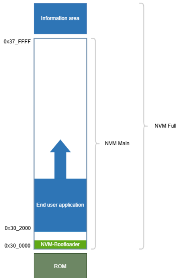
Figure 10-7: Minimalistic NVM layout content
