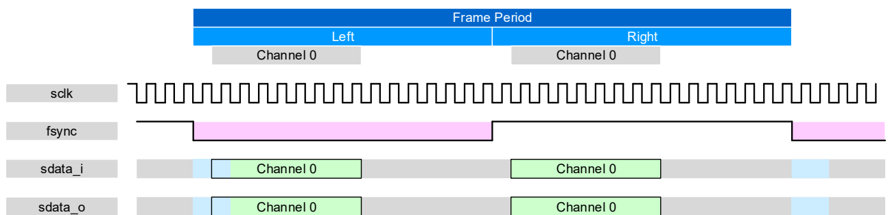
Figure 8-10: I2S frame format
