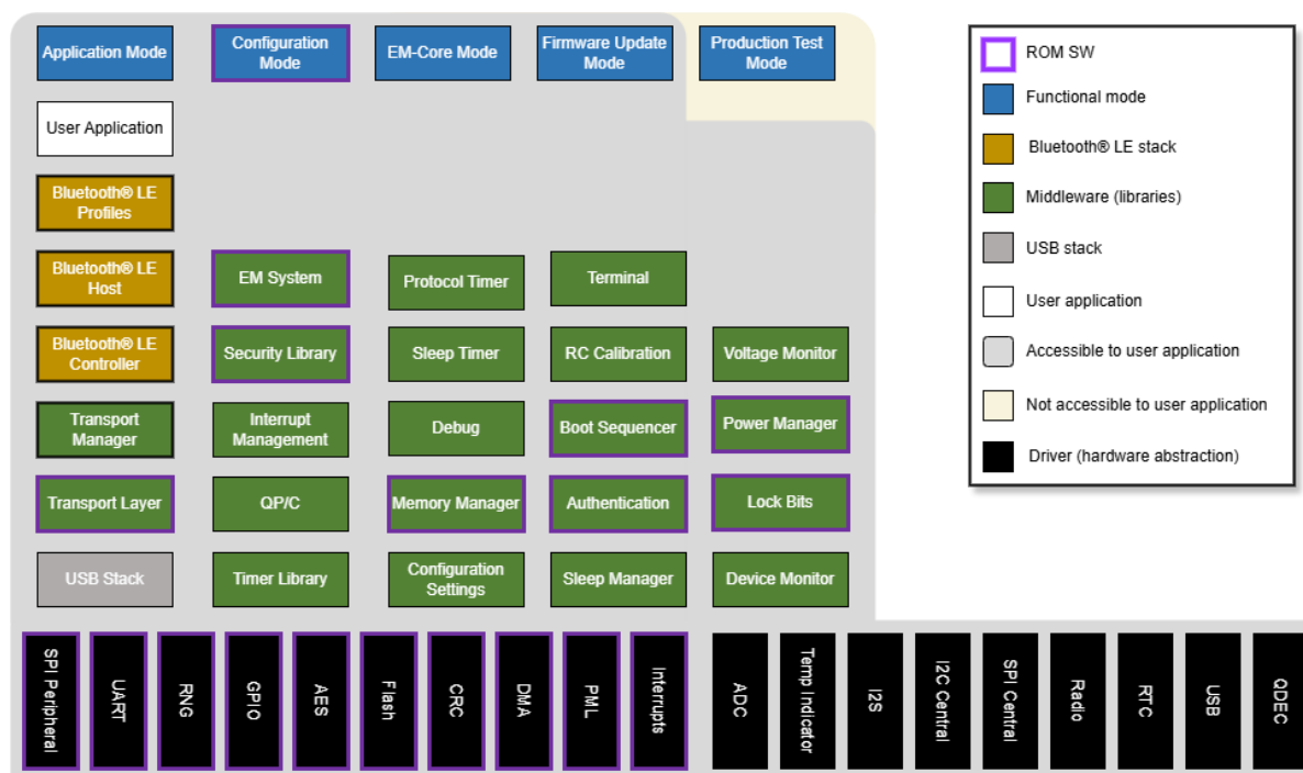
Figure 10-1: Software architecture
