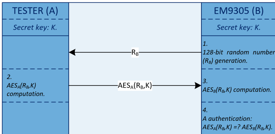
Figure 9-4: AES-based two-pass authentication
