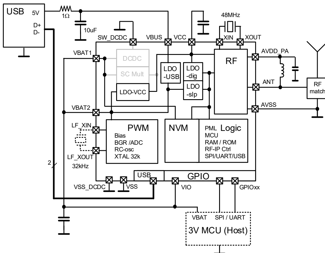
Figure 1-7: USB configuration
