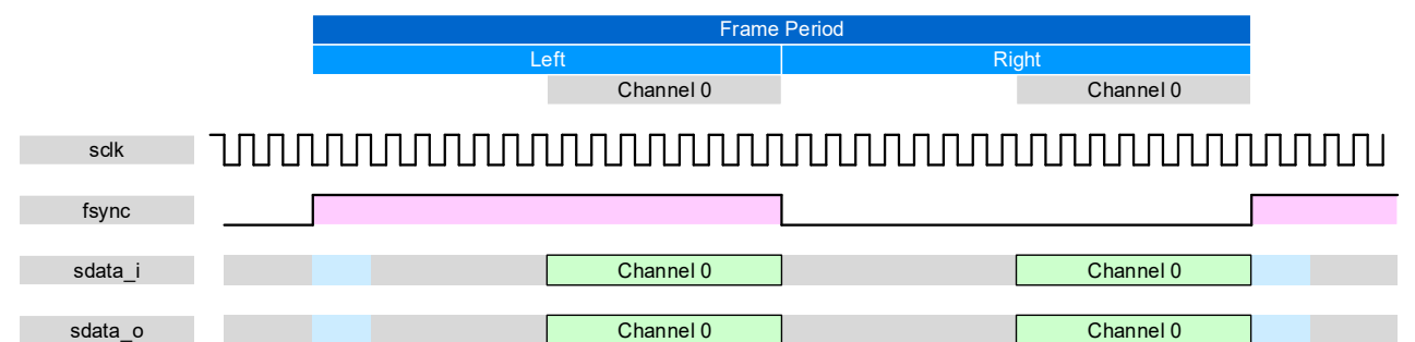
Figure 8-12: Right-Justified frame format
