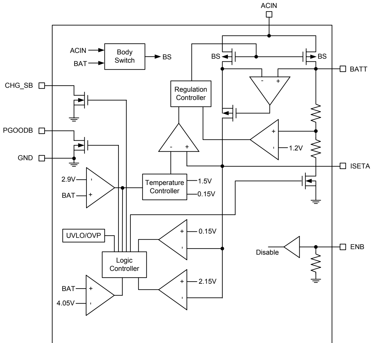
FIG.1. Functional Block Diagram of EMC5045
