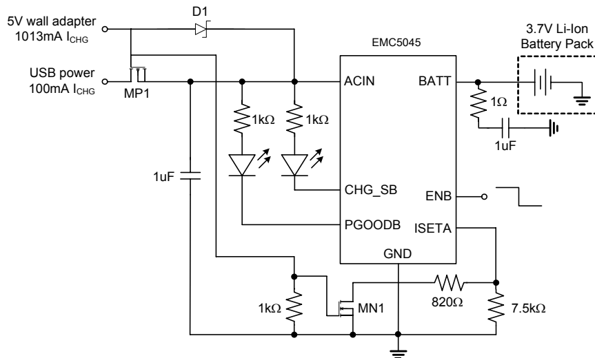
FIG.7. Combining wall adapter and USB power
