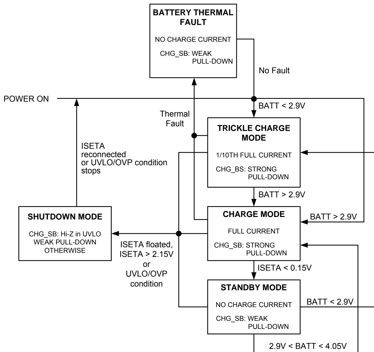
FIG.2. EMC5045 flow chart
