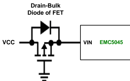
FIG.6. Low loss input reverse polarity protection
