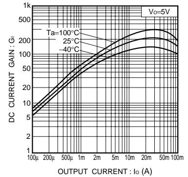
Fig.11 DC current gain vs. output current
