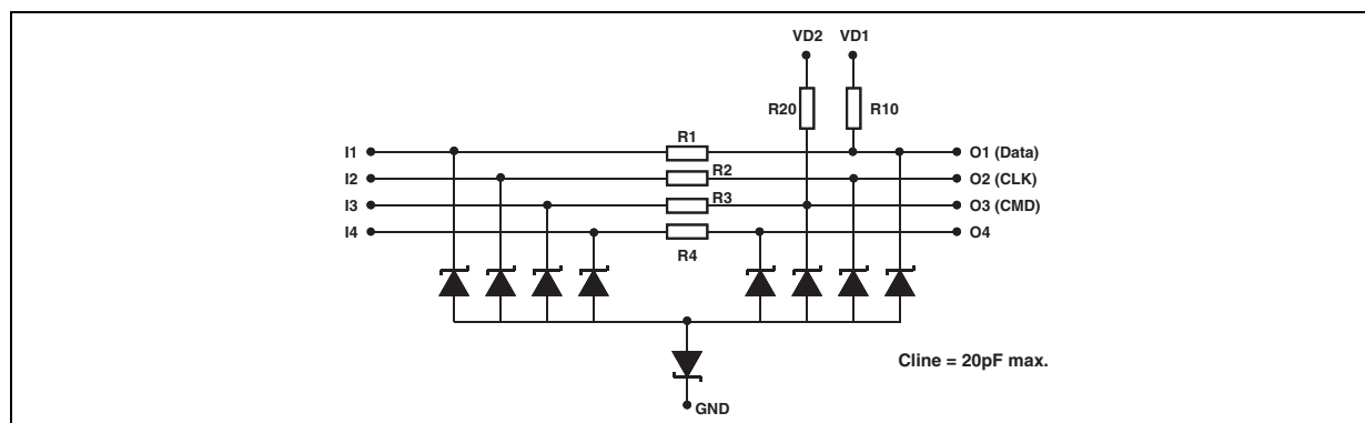
Figure 2: Configuration
