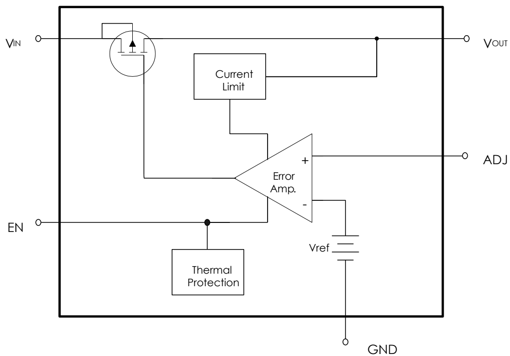
FIG.1. Functional Block Diagram of EMP8045
