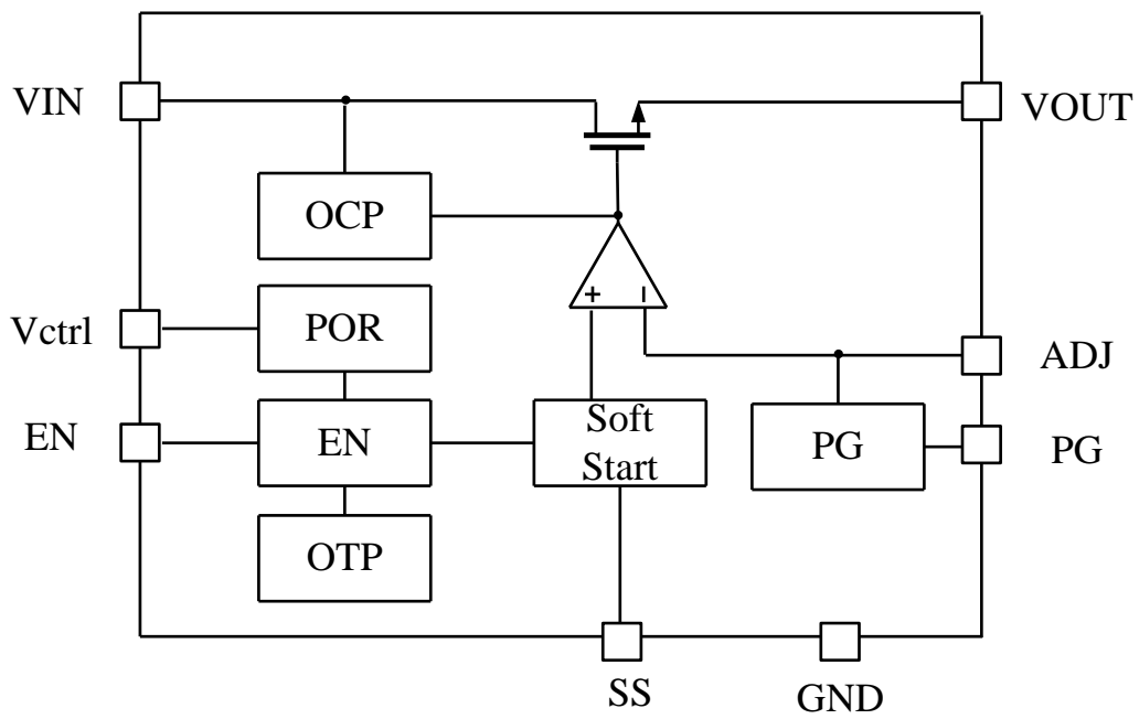
FIG.1. Functional Block Diagram of EMP8165/A
