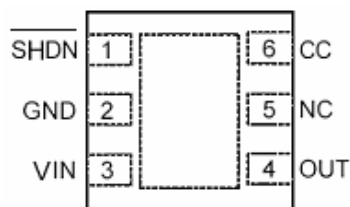
TDFN-6(TOP VIEW)
