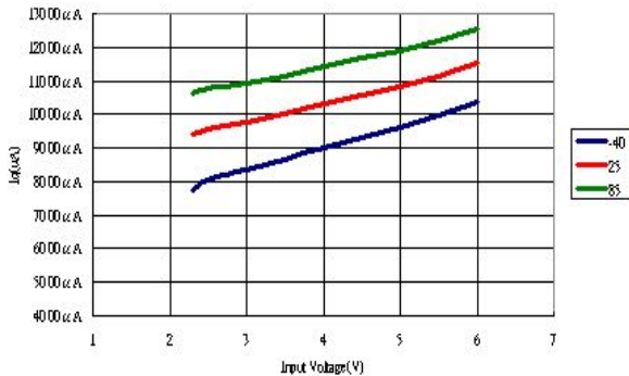
CH2 Supply Current vs. Input Voltage
