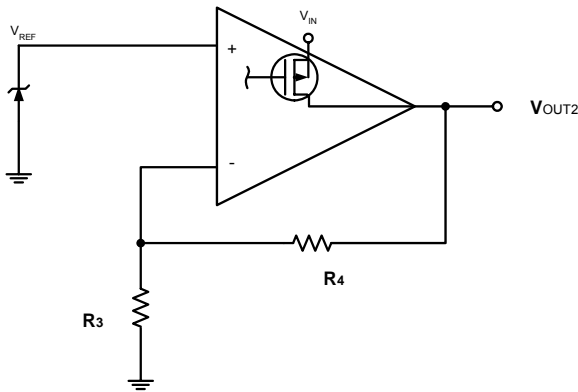
Figure 3. Simplified Regulator Topology
