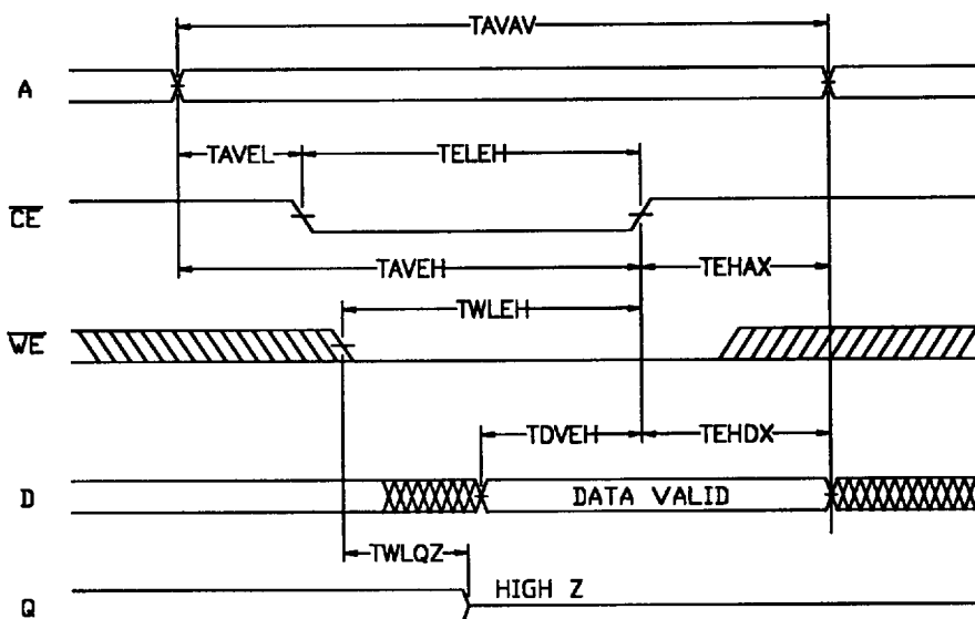
Write Cycle 2: \overline{CE} Control
