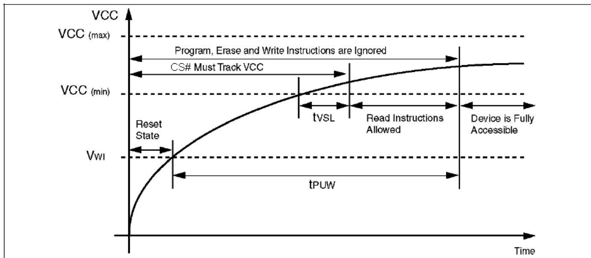
Figure 31. Power-up Timing
