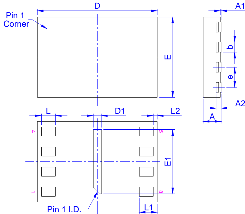
Figure 39. USON (8L 2x3x0.45mm)
