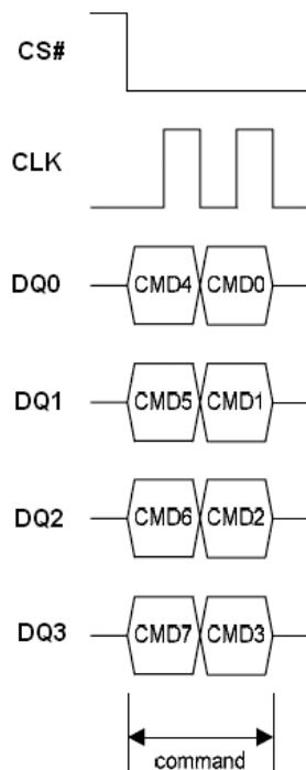
Figure 9.1 Write Enable/Disable Instruction Sequence in QPI Mode
