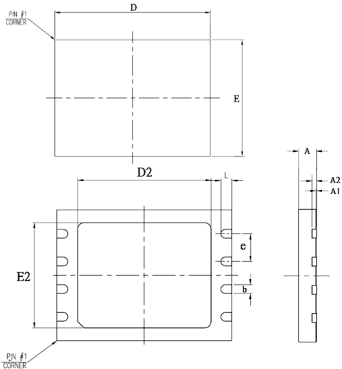
Figure 40. VDFN8 ( 5x6mm )
