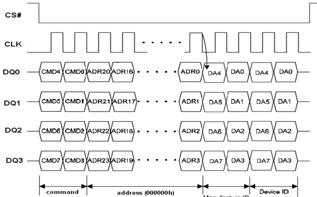
Figure 27.1. Read Manufacturer / Device ID Diagram in QPI Mode
