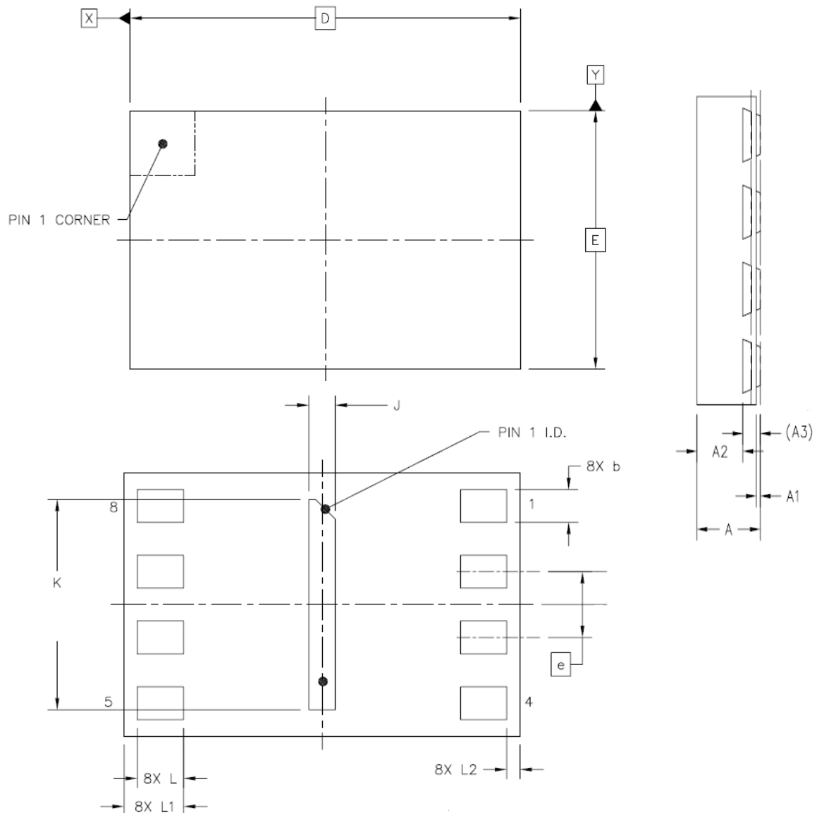
Figure 38. USON (8L 2x3x0.55mm)
