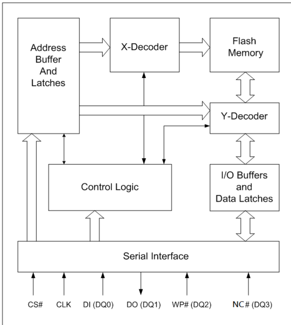
Figure 2. BLOCK DIAGRAM
