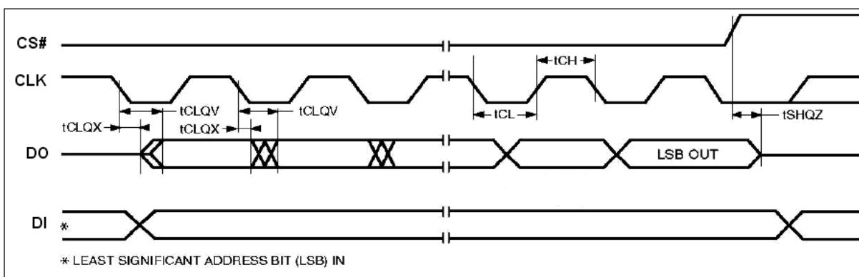
Figure 35. Serial Output Timing
