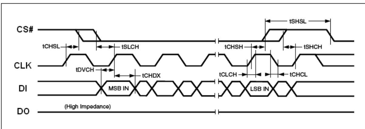
Figure 36. Input Timing
