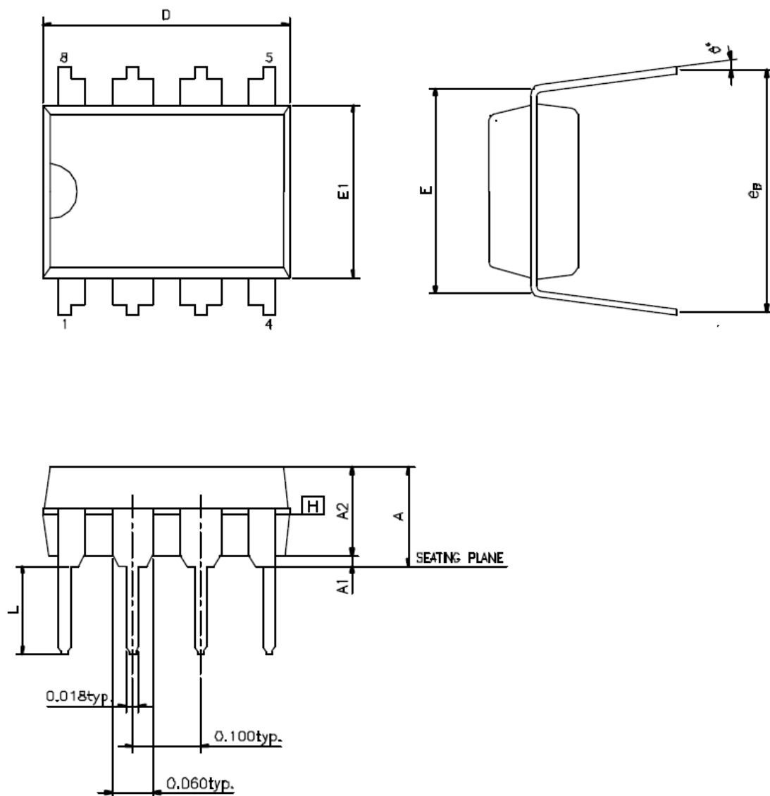
Figure 41. PDIP8
