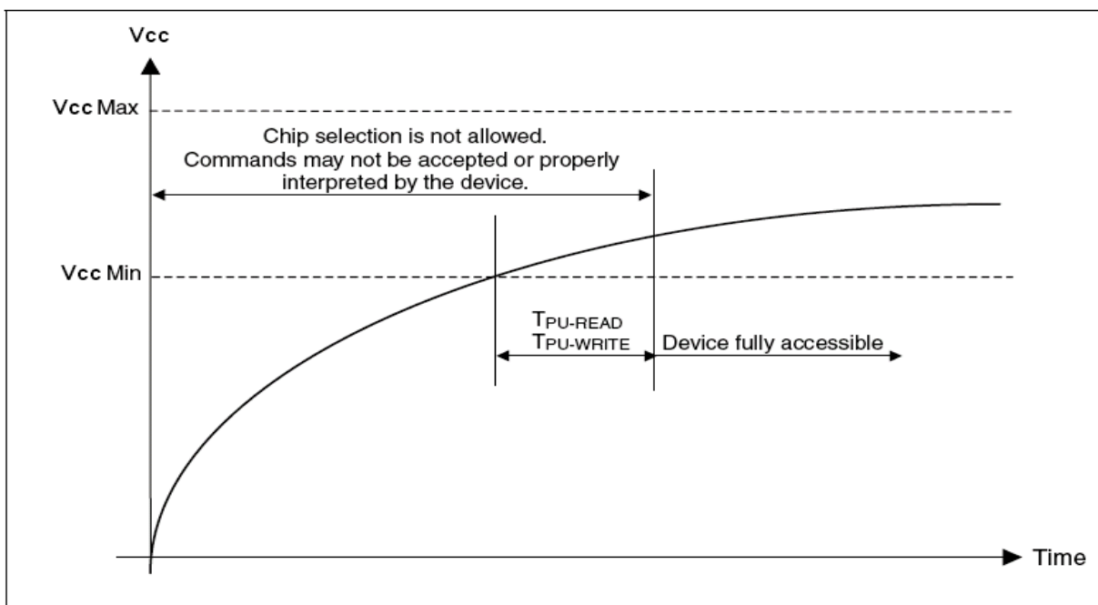
Figure 33. Power-up Timing
